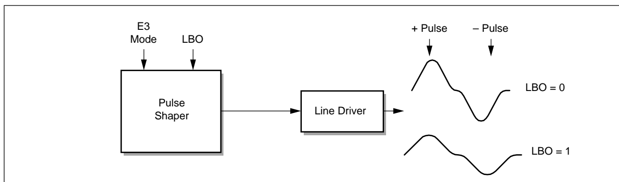
Figure 2-2. Pulse Shaper
