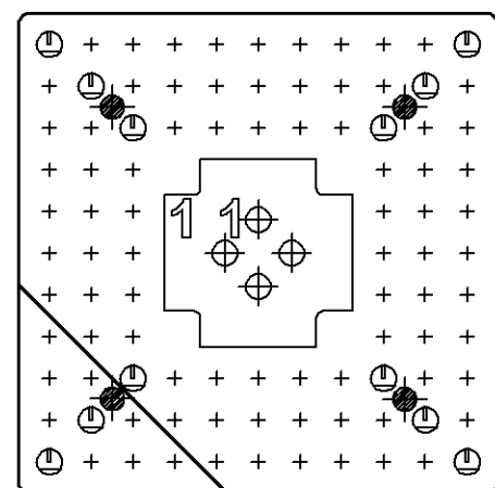
1-55271-2 96 POSITION
