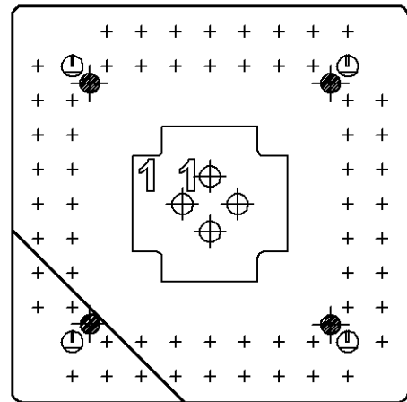
55271-1 65 POSITION
