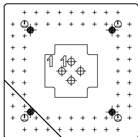
55271-4, 1--1 68 POSITION
