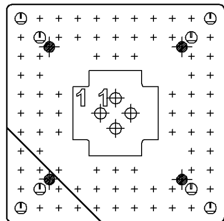
55271-3,-6 85 POSITION
