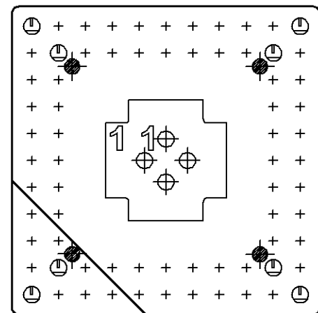
1-55271-0 72 POSITION
