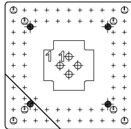
1-55271-3 73 POSITION
