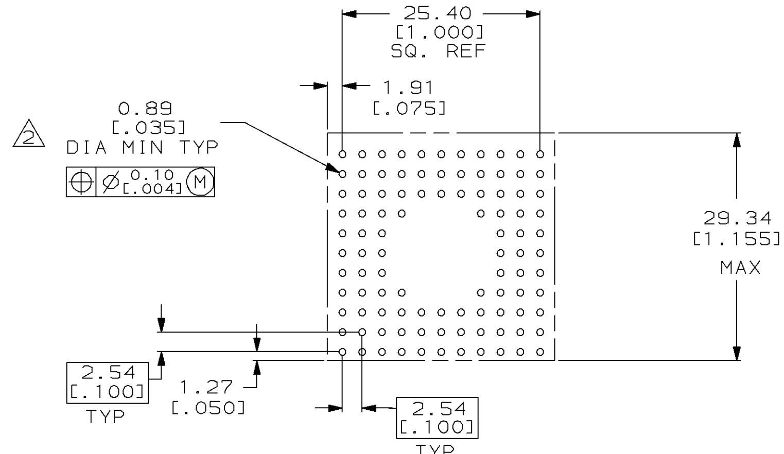
RECOMMENDED P.C. BOARD PATTERN
