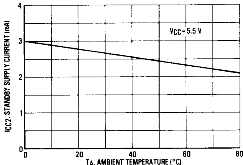
FIGURE 14 — I_{CC2} STANDBY CURRENT versus AMBIENT TEMPERATURE
