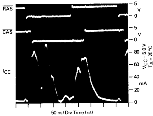
FIGURE 20 — \overline{\text{RAS}}/\overline{\text{CAS}} CYCLE
