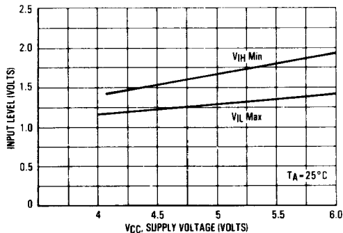
FIGURE 16 — ADDRESS INPUT LEVEL versus SUPPLY VOLTAGE
