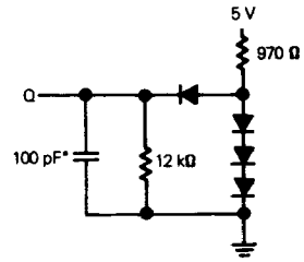
FIGURE 1 — OUTPUT LOAD
