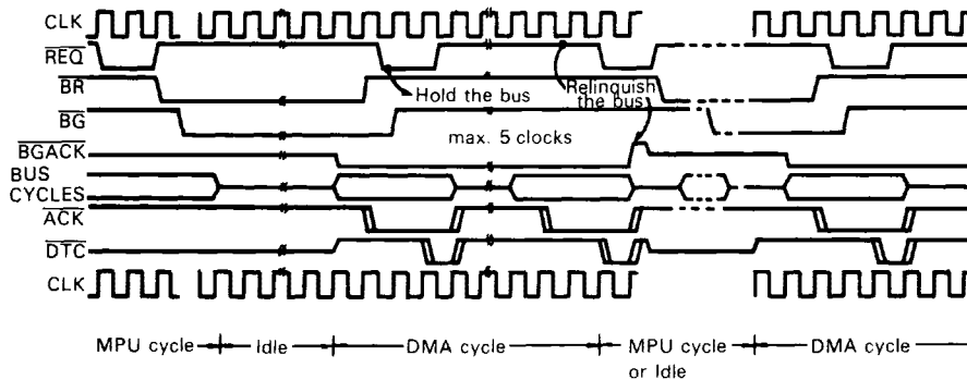
Figure 17 Cycle Steal Mode Request Timing
