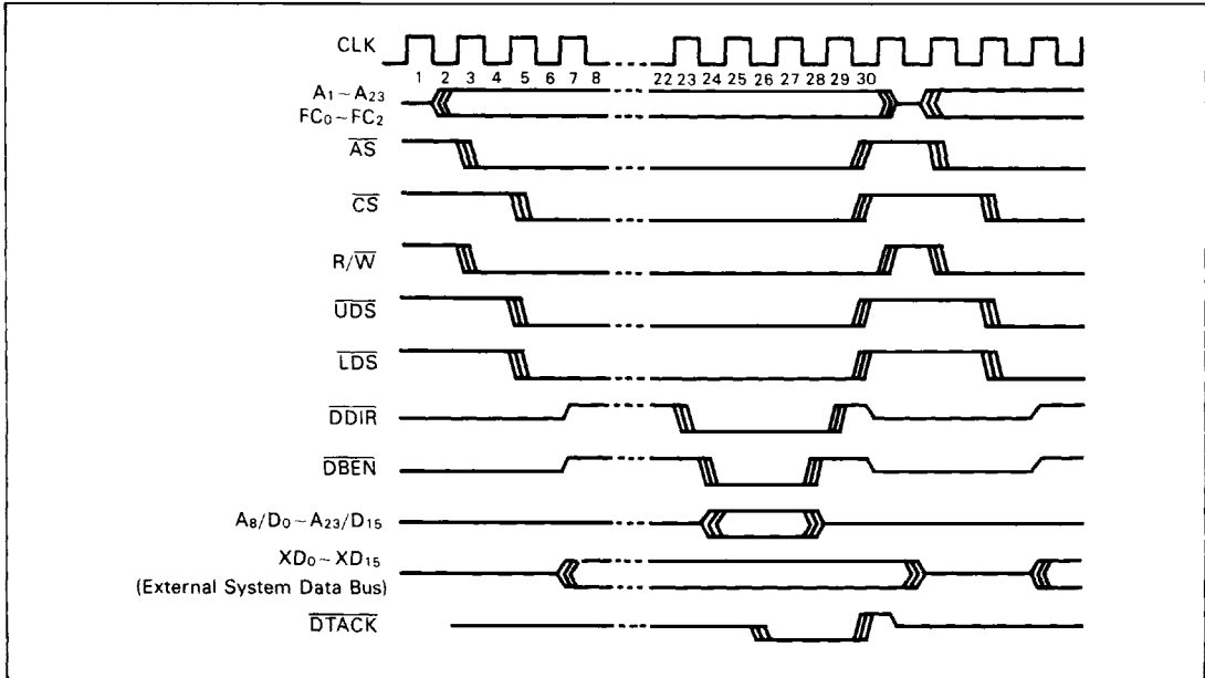
Figure 13 MPU Write to DMAC-Word
