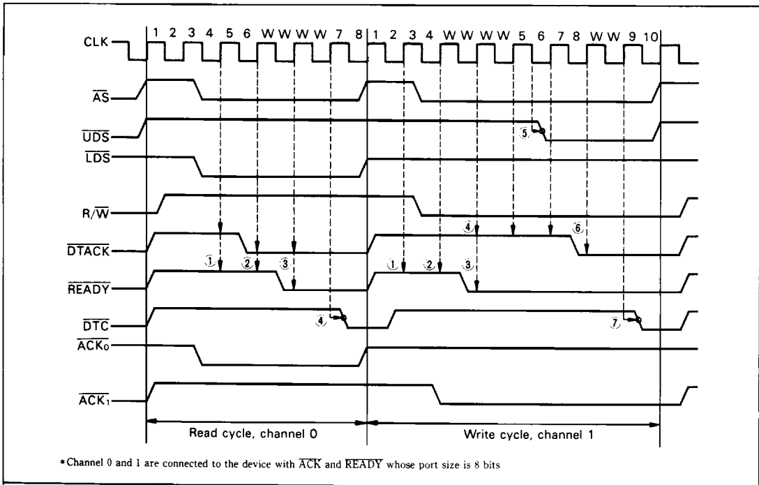
Figure 33 Device with \overline{\text{ACK}} and \overline{\text{READY}} Mode Timing
