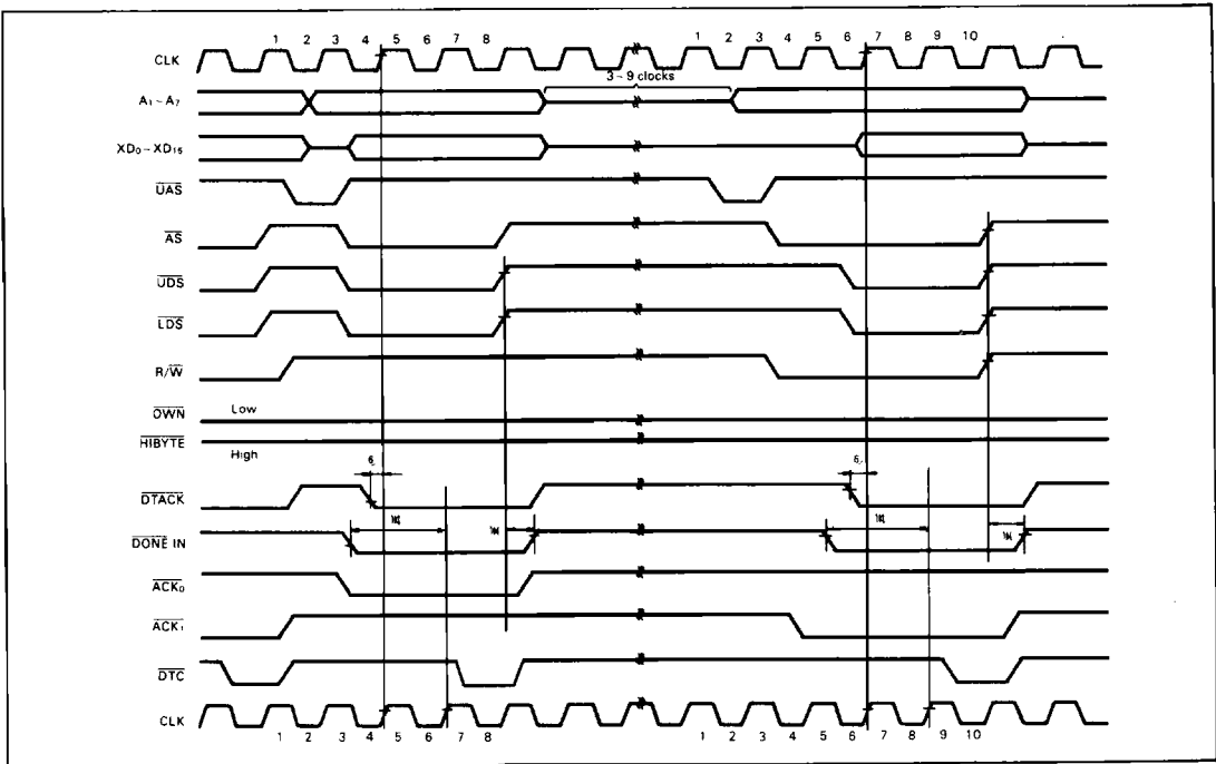
Figure 8 AC Electrical Waveforms- \overline{DONE} Input
