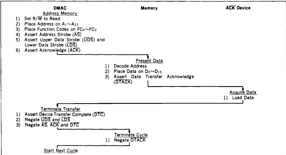
Figure 28 Word from Memory to Device with \overline{ACK}
