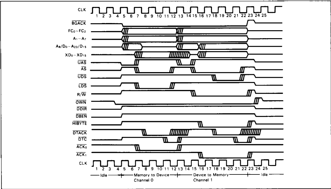
Figure 30 Single Addressing Mode with 8-Bit Devices as Source and Destination (Read-Write Cycles)
