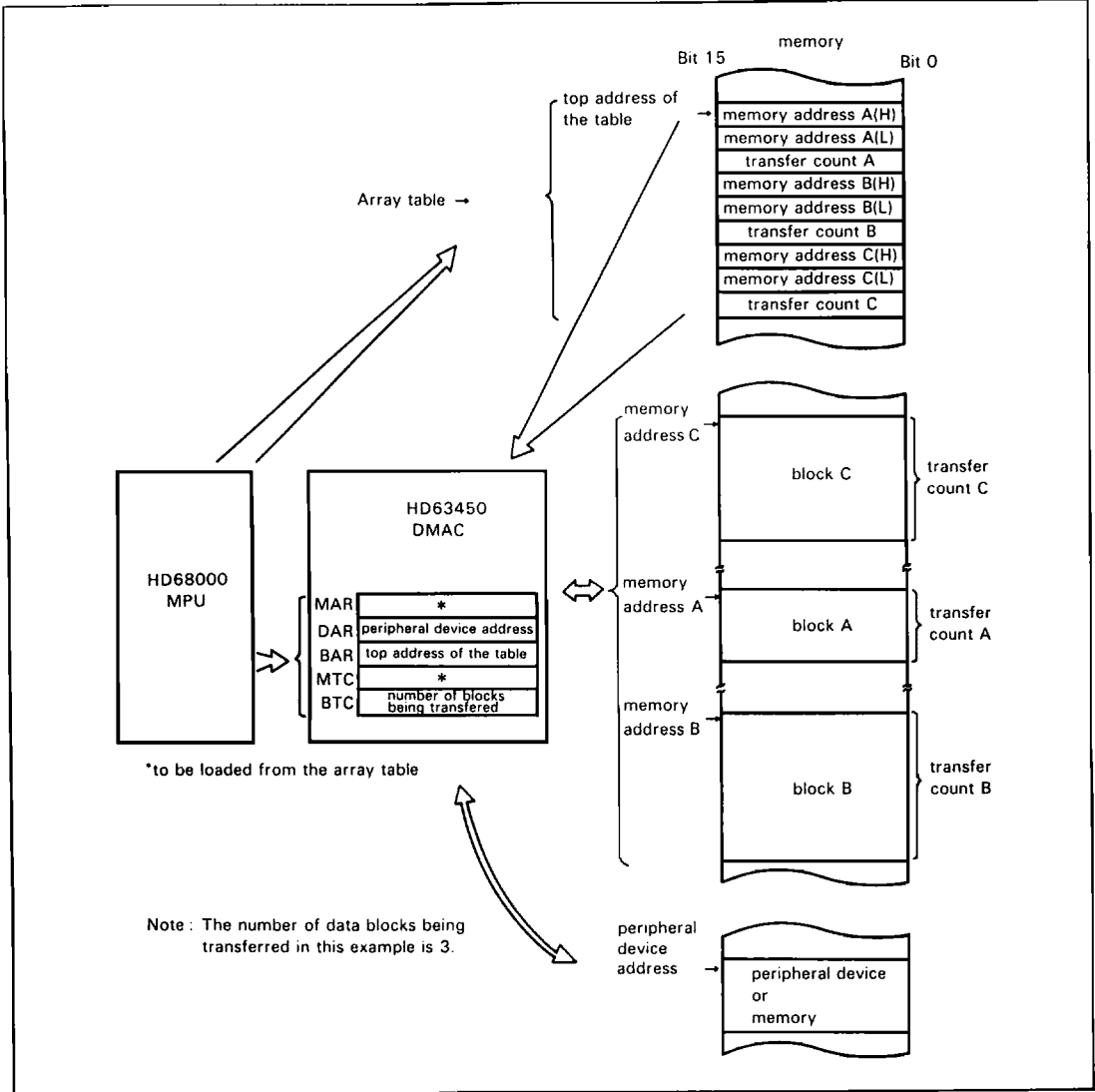
Figure 38 Transfer Example of the Array Chaining Mode
