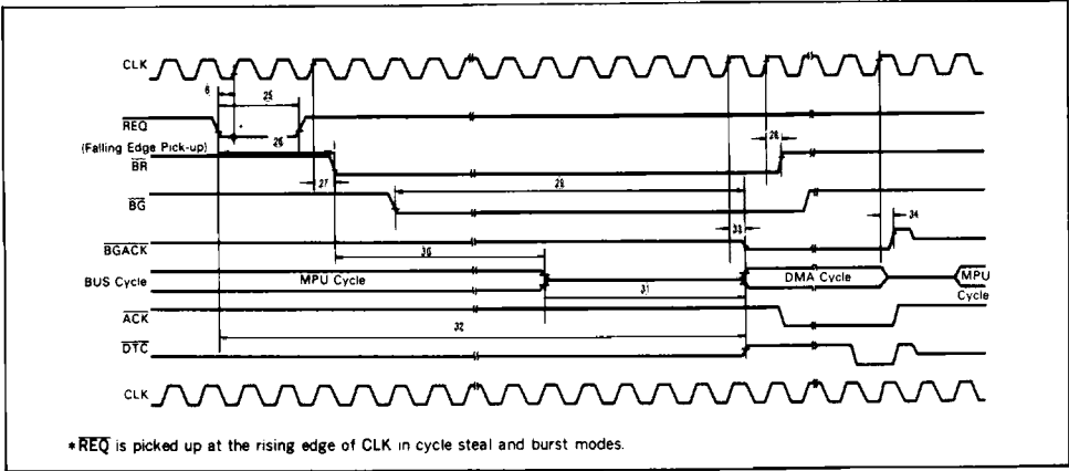
Figure 4 AC Electrical Waveforms-Bus Arbitration
