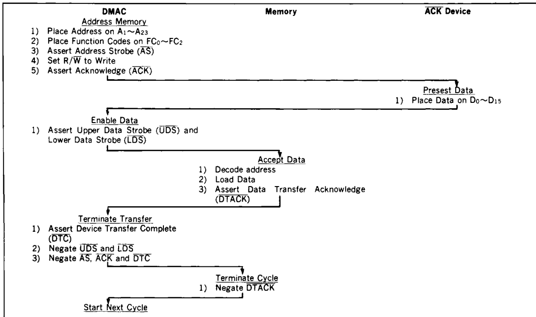
Figure 29 Word from Device with \overline{ACK} to Memory
