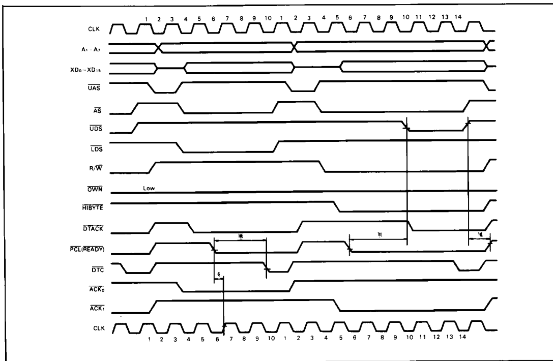
Figure 7 AC Electrical Waveforms-DMA Read/Write (Single Cycle with \overline{\text{ACK}} and \overline{\text{READY}} )
