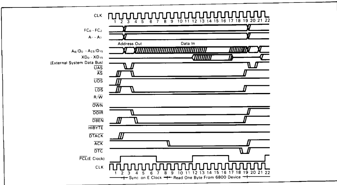
Figure 26 Dual Addressing Mode, HD6800 Compatible Device, Read Cycle
