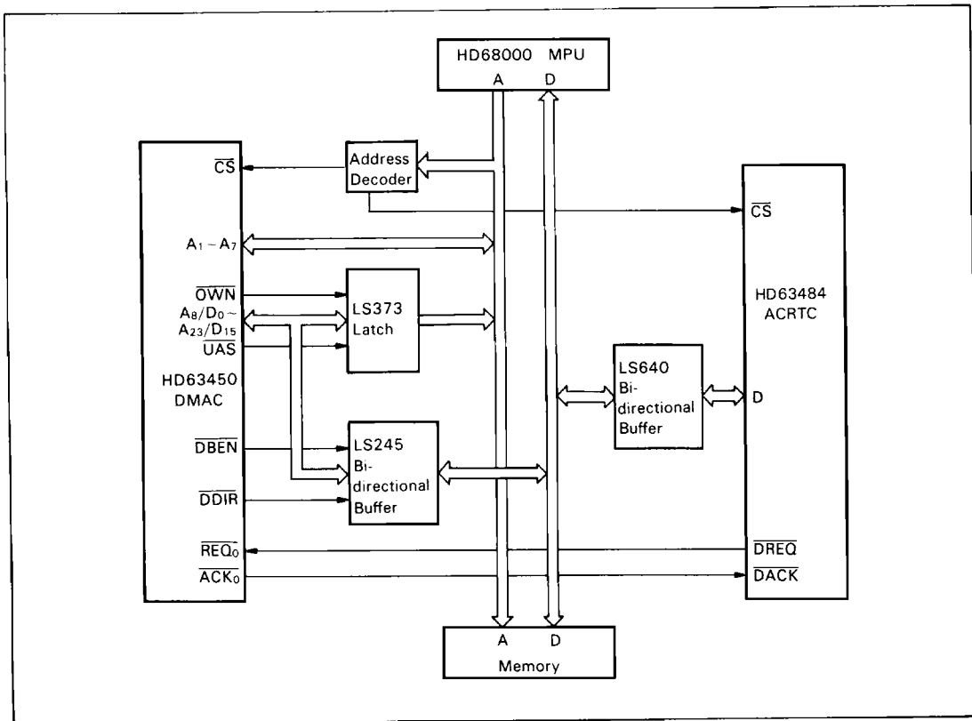
Figure 9 Typical System Configuration
