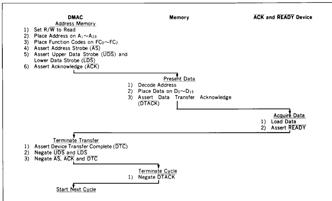
Figure 34 Word from Memory to Device with \overline{ACK} and \overline{READY}
