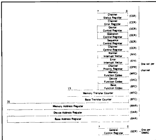
Figure 11 Internal Registers
