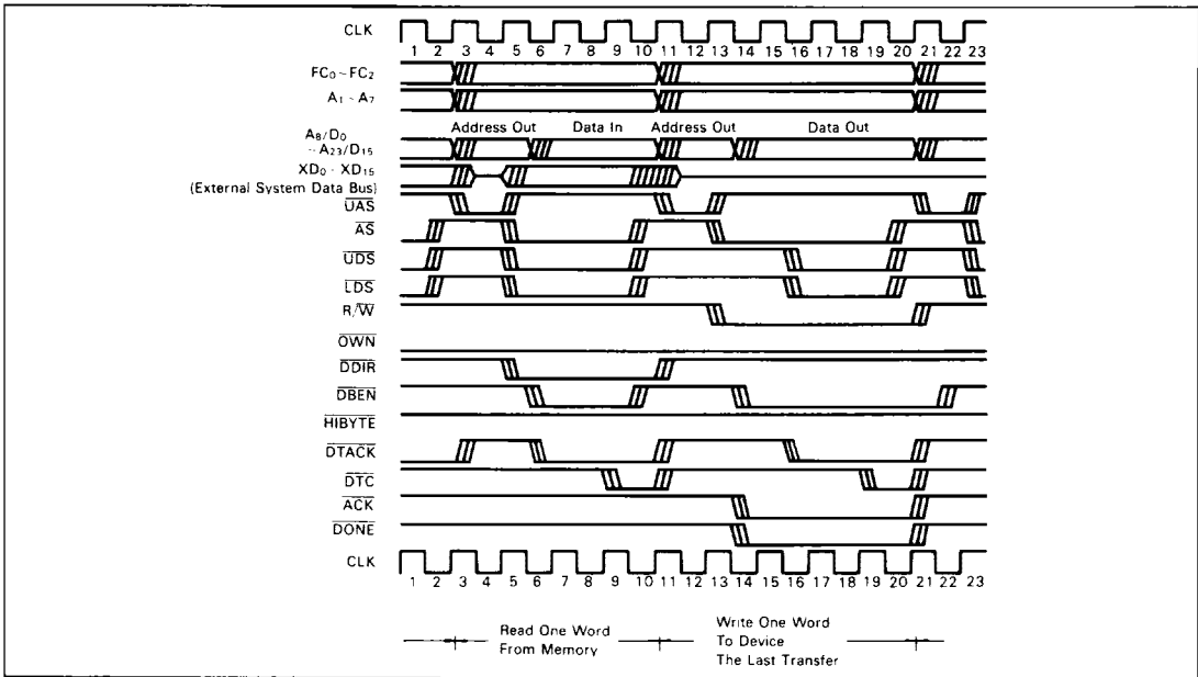
Figure 21 Dual Addressing Mode, Read/Write Cycle, Destination=16-bit Device, Word Operand
