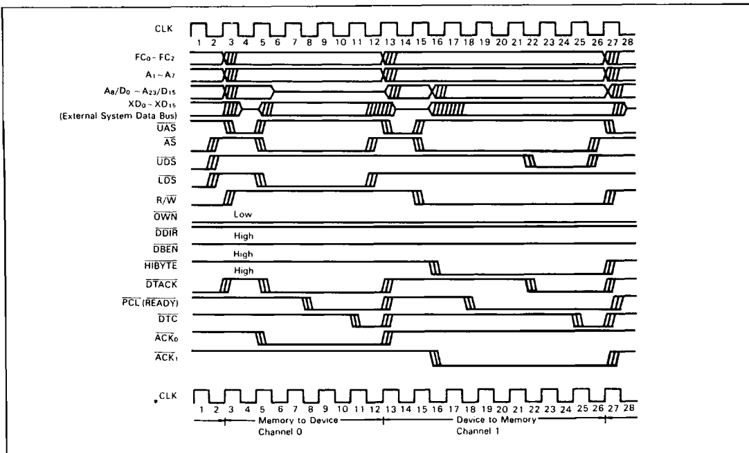
Figure 36 Single Addressing Mode with 8-bit Device as Source and Destination with PCL Used as a READY input (Read-Write Cycles)
