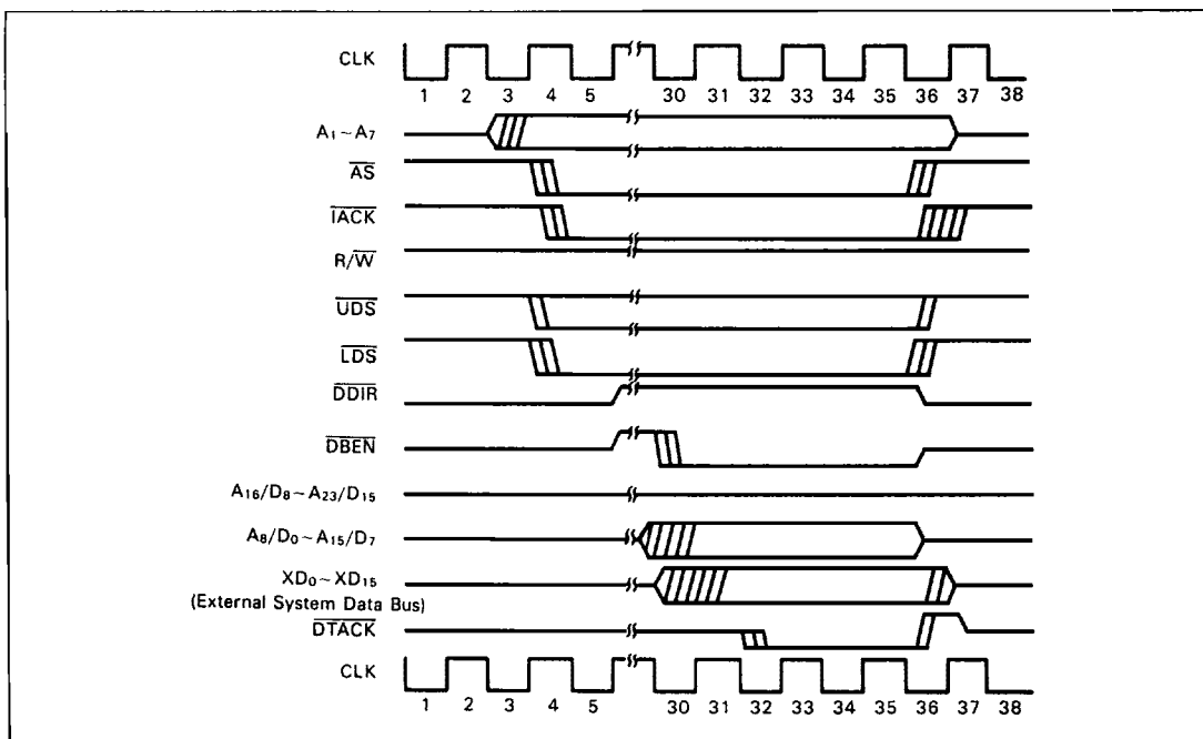
Figure 37 MPU \overline{IACK} Cycle to DMAC
