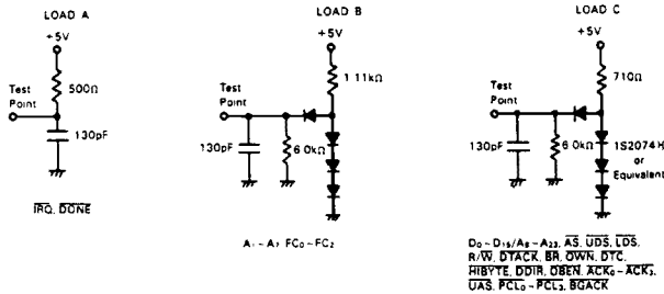
Figure 1 Test Loads
