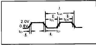
Figure 2 Input Clock Waveform
