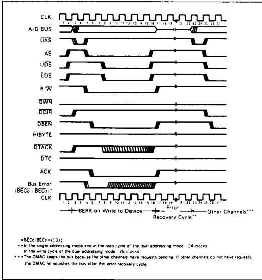
Figure 41 Bus Error Operation
