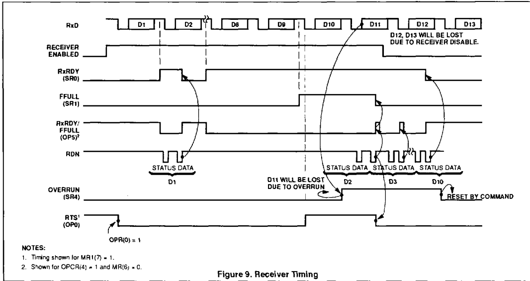
Figure 9. Receiver Timing
