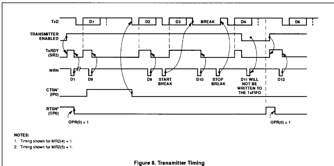
Figure 8. Transmitter Timing
