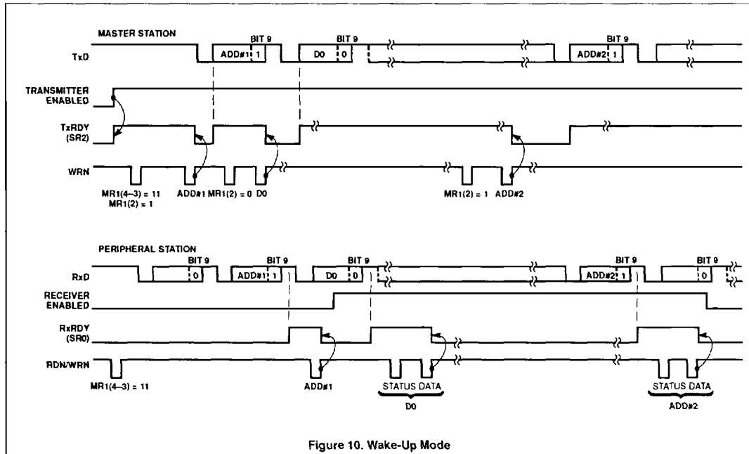
Figure 10. Wake-Up Mode
