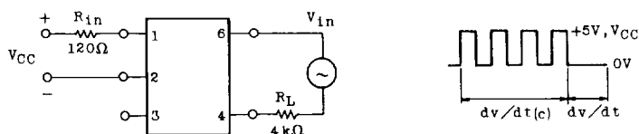
Fig. 1 dv/dt TEST CIRCUIT
