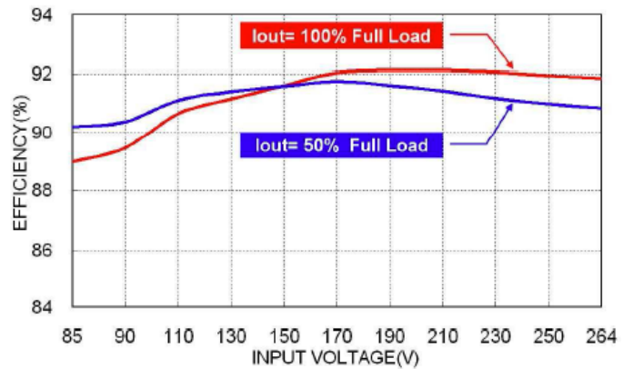
Efficiency vs. Input Voltage PSMAD40-24S-U
