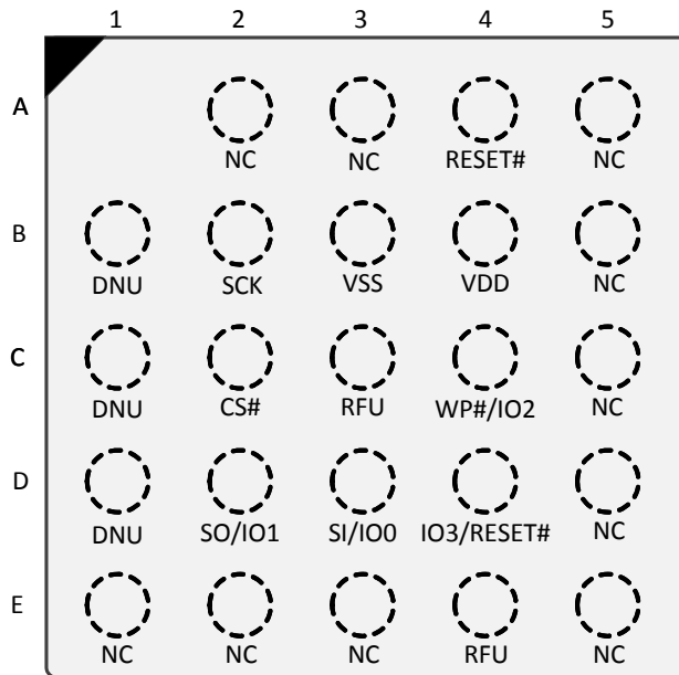
Figure 6.4 24-Ball BGA, 5x5 Ball Footprint (FAB024), Top View
