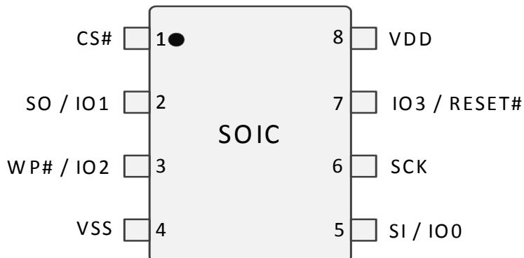
Figure 6.2 8-Pin Plastic Small Outline Package (SOIC8)
