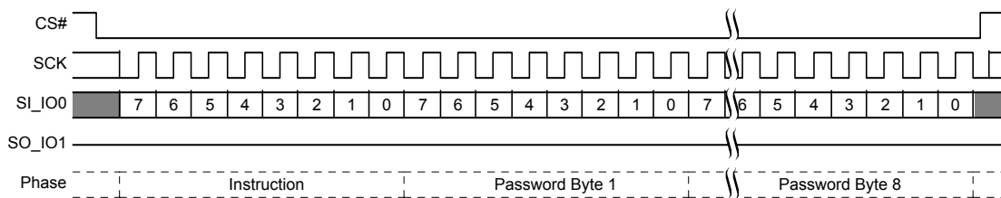
Figure 9.93 Password Unlock (PASSU) Command Sequence
