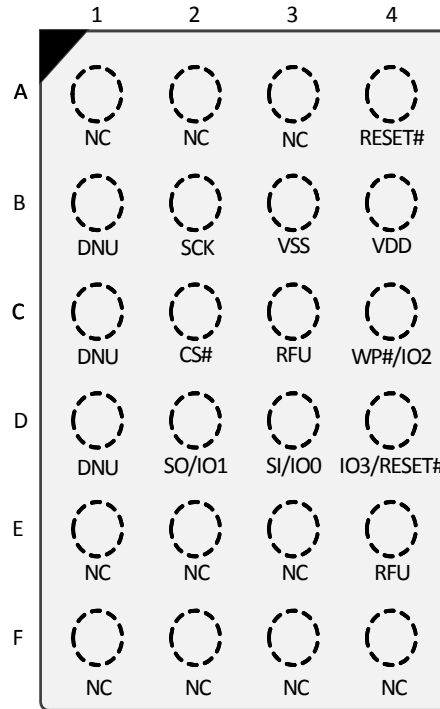
Figure 6.5 24-Ball BGA, 4x6 Ball Footprint (FAC024), Top View
