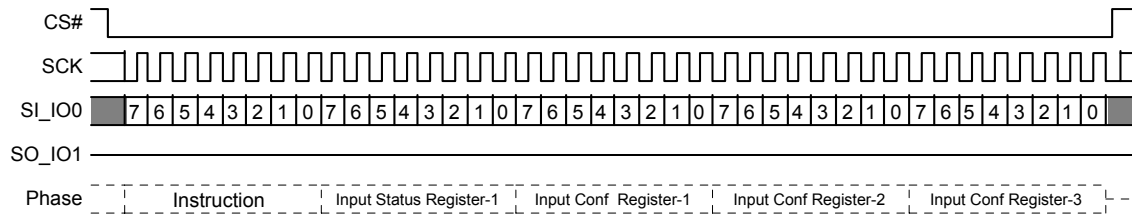
Figure 9.13 Write Registers (WRR) Command Sequence
