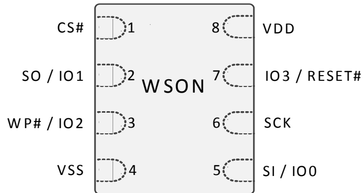
Figure 6.3 8-Connector Package (WSON 6x8) (WSON 5x6), Top View
