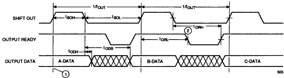
Figure 4. Output Timing
