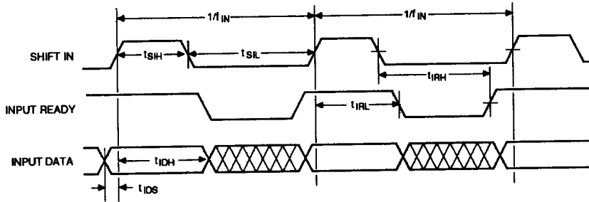
Figure 1. Input Timing
