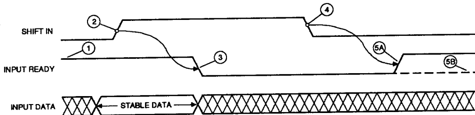
Figure 1. Input Timing
