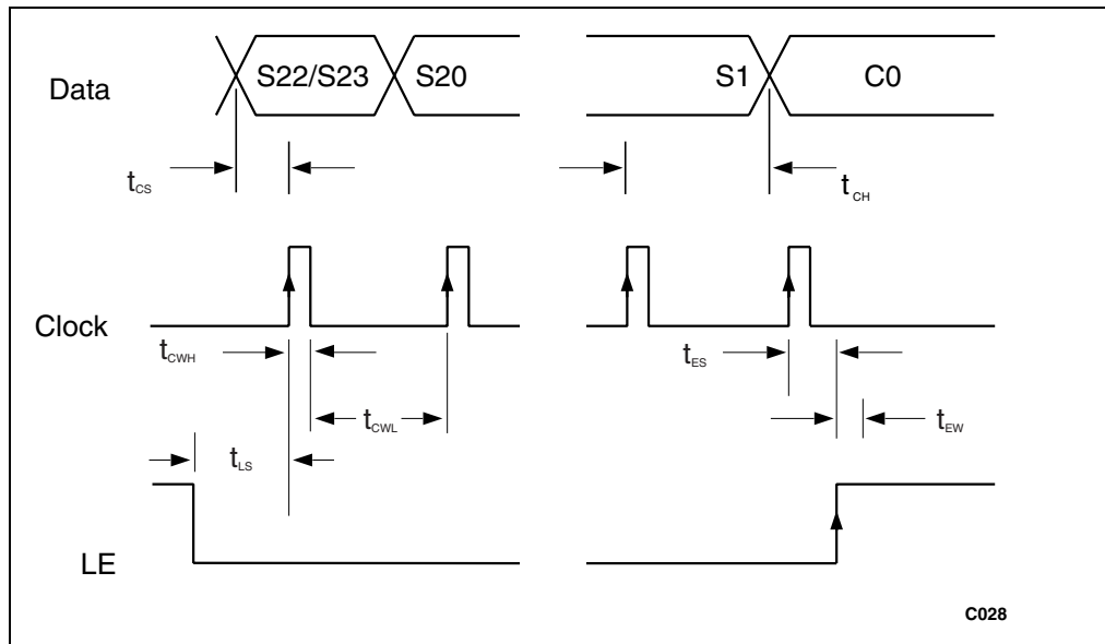
Figure 6. CX74016 Timing Diagram
