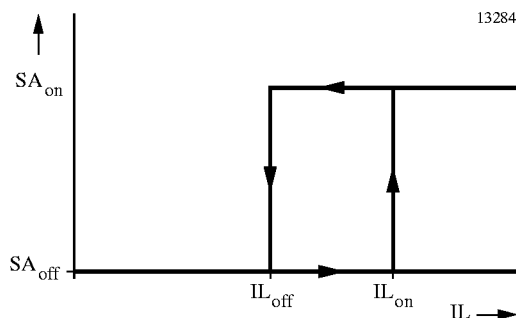
Figure 11. Threshold of speaker amplifier
