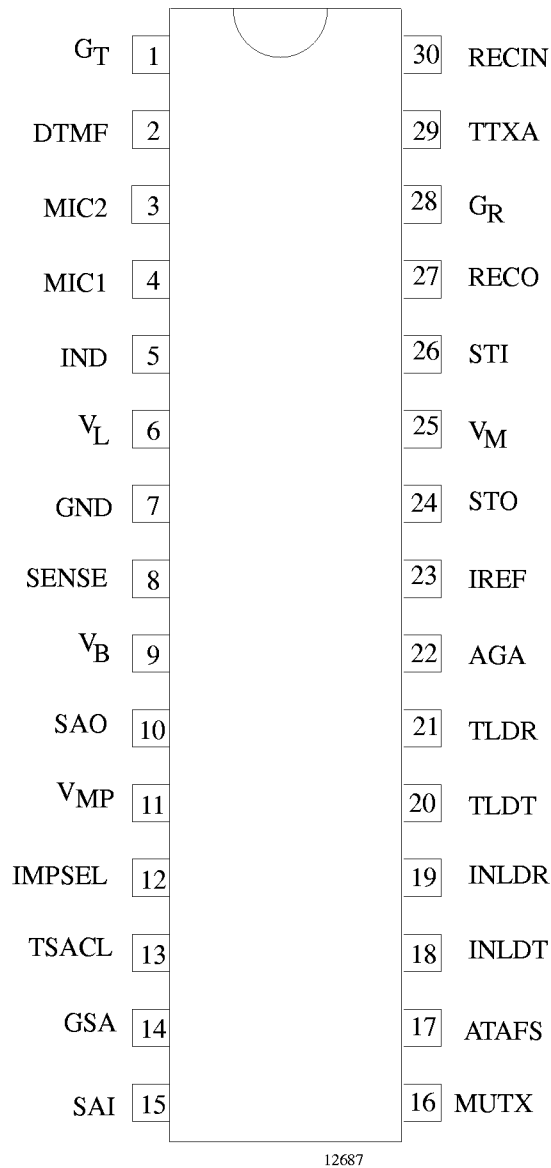
Figure 3. Pinning SDIP30
