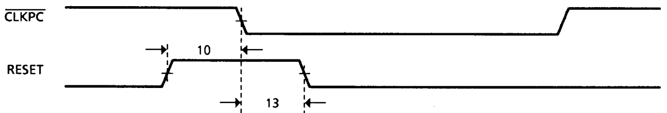
Figure 8. RESET Timing
