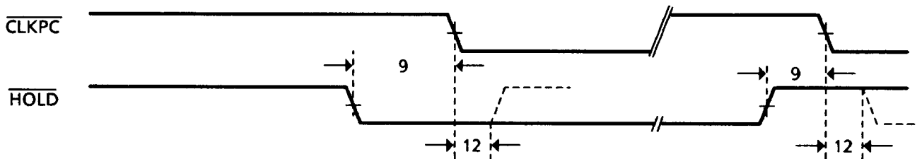
Figure 9. HOLD Timing
