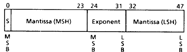
Figure 4. Data Formats
