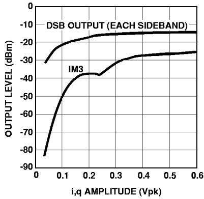
Figure 19. Modulator + Mixer DSB Performance vs. i,q Amplitude (Each Pin, Referenced to Ground).
