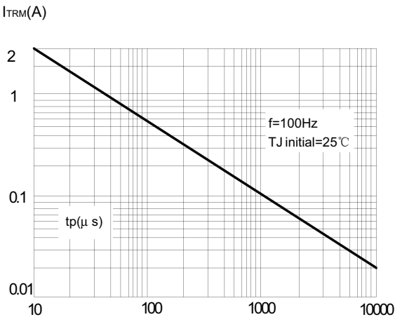
FIG.6-PEAK PULSEE CURRENT VERENT VERSUS PULSE DURATION(MAXIMUM VALUES)
