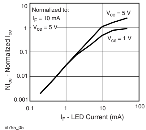
Fig. 5 - Normalized Non-Saturated and Saturated Collector-Emitter Current vs. LED Current
