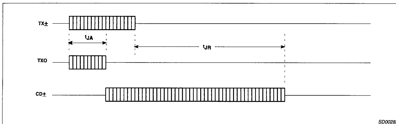
Figure 8. Jabber Timing
