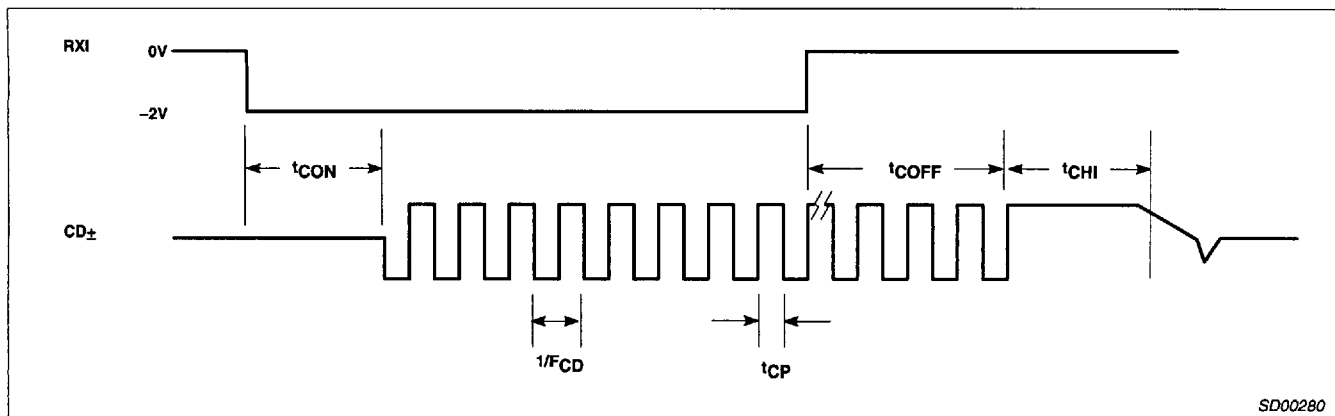
Figure 6. Collision Timing
