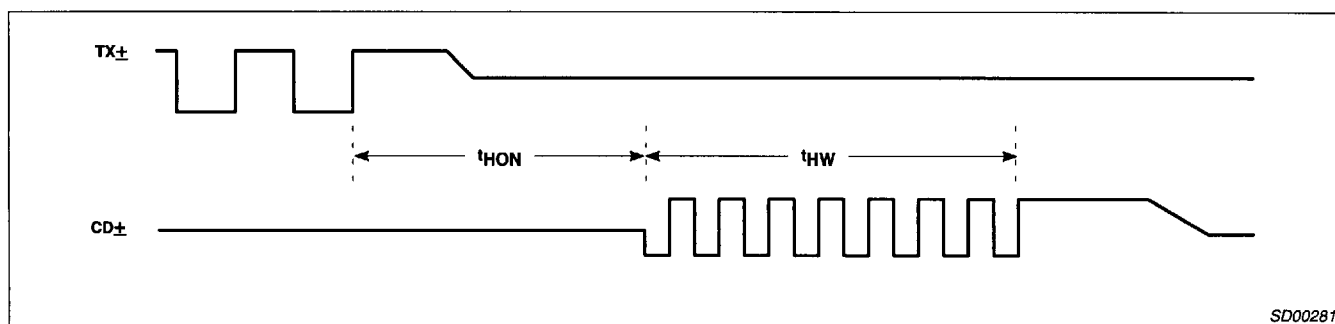
Figure 7. Heartbeat Timing
