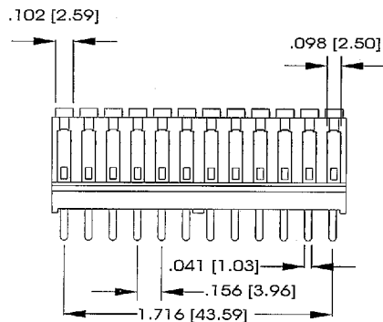
MTG Housing
