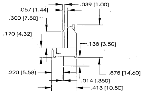
MTGC Contact
