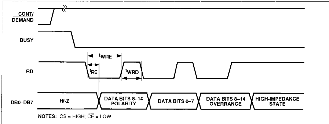
Figure 12 Bus Output Timing, Continuous Mode
