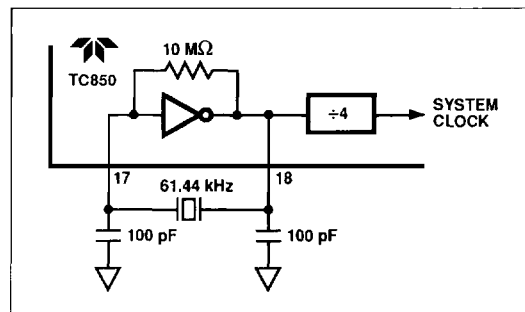
Figure 6 Crystal Oscillator Schematic
