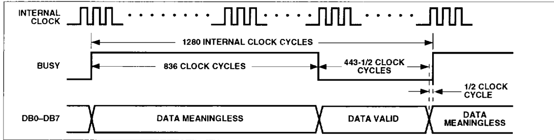
Figure 11 Conversion Timing, Continuous Mode
