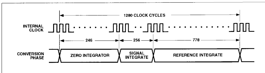
Figure 4 Conversion Timing
