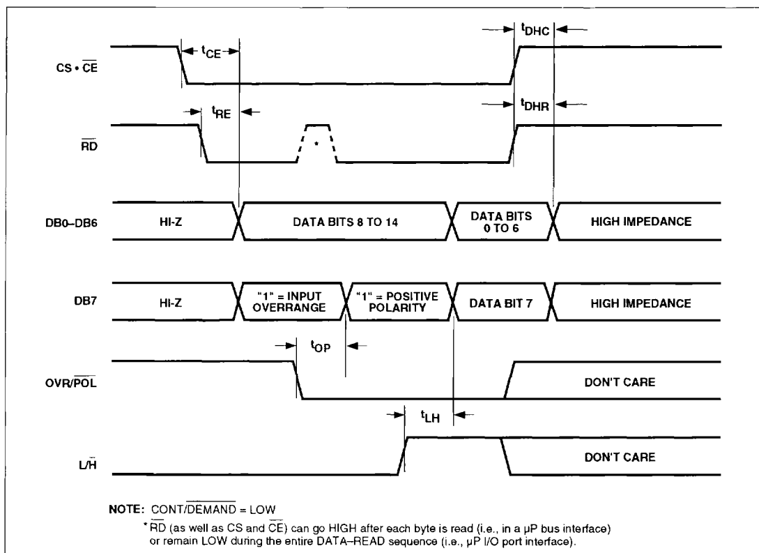
Figure 10 Bus Output Timing, Demand Mode
