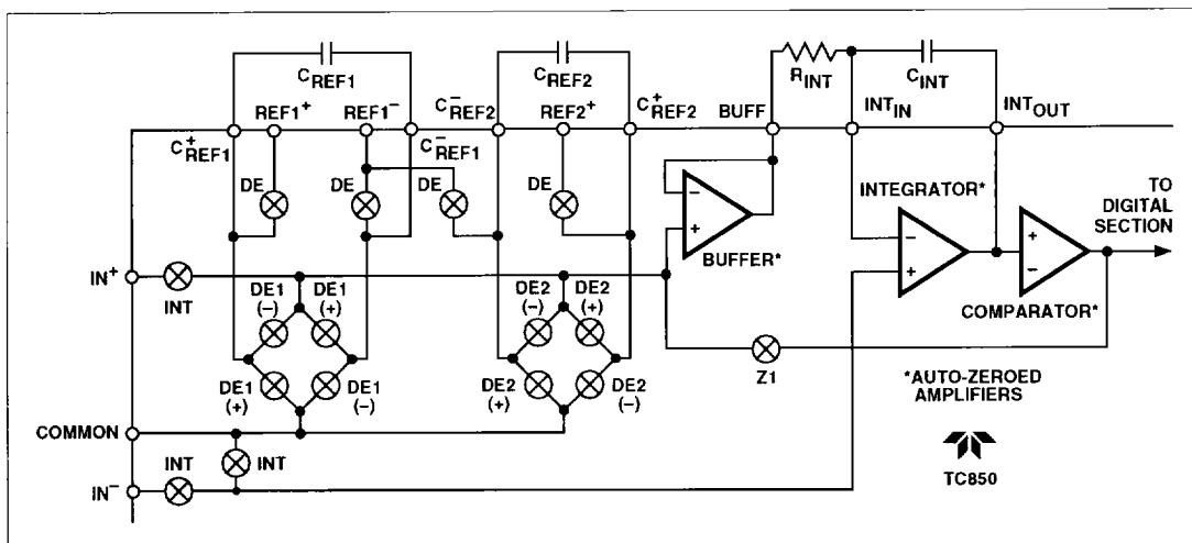
Figure 3 Analog Section Simplified Schematic
