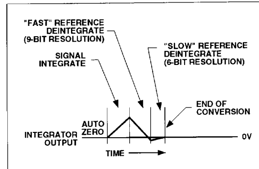
Figure 2B "Fast-Slow" Reference Deintegrate Cycle
