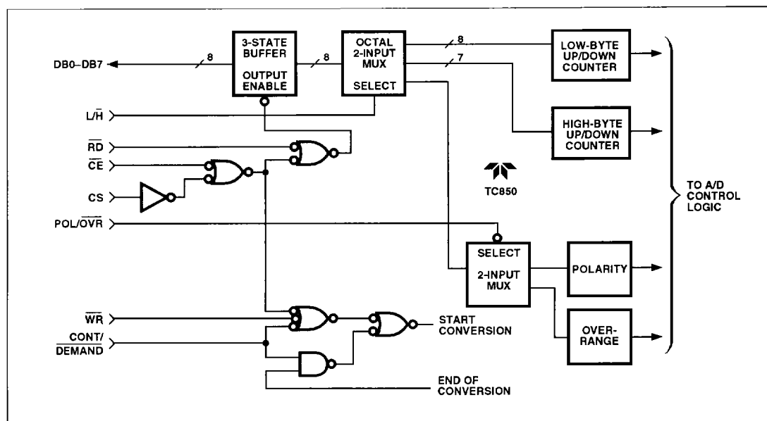
Figure 5 Bus Interface Simplified Schematic
