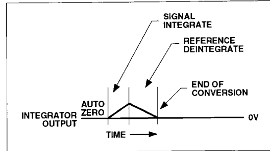
Figure 2A Dual-Slope ADC Cycle
