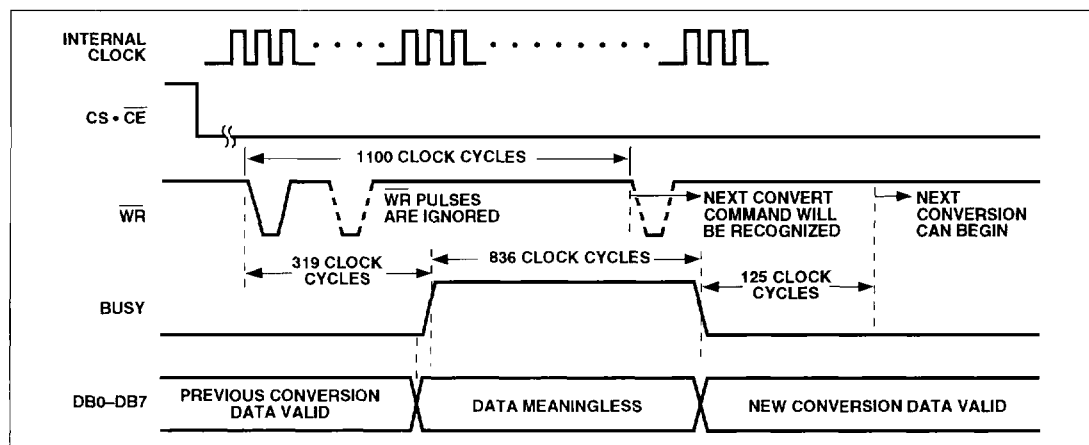
Figure 9 Conversion Timing, Demand Mode
