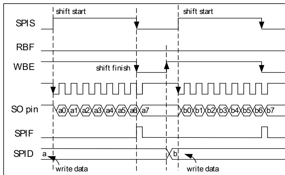
Fig. 5-14 Transmit Mode (8-bit, 1 word)
