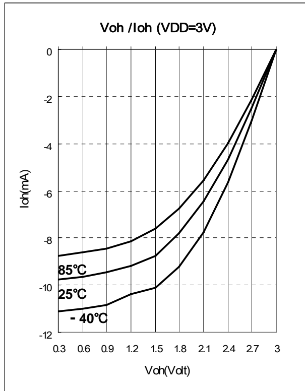
Fig. 7-3 Port 6, Port 7, Port 8 and Port 9 Voh vs. Ioh, VDD=3V
