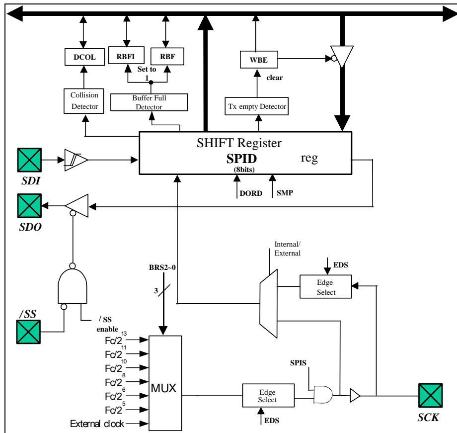
Fig. 5-13 SPI Block Diagram
