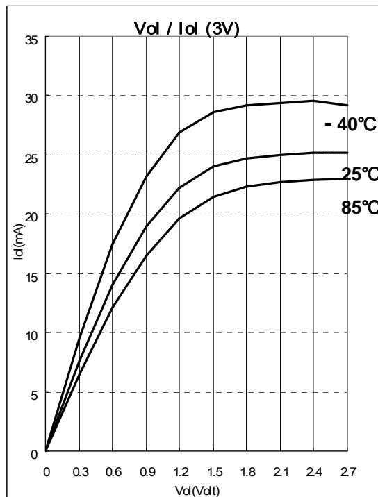
Fig. 7-5 Port 6, Port 7 and Port 8 Vol vs. Iol, VDD=3V
