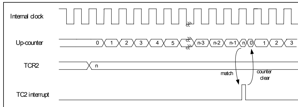
Fig. 5-19 Timer Mode Timing Chart
