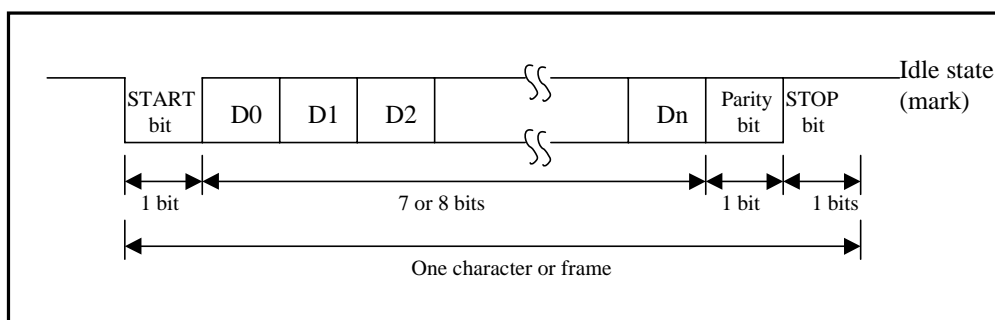
Fig. 5-11 Data Format in UART
