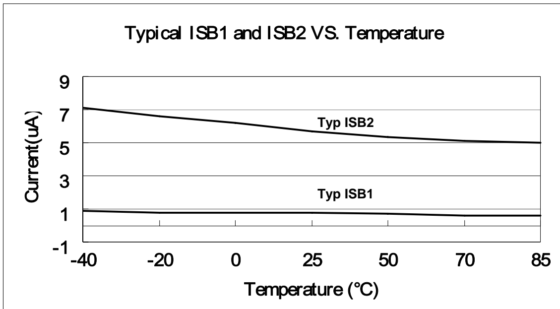
Fig. 7-15 Typical Standby Current (ISB1 and ISB2) vs. Temperature
