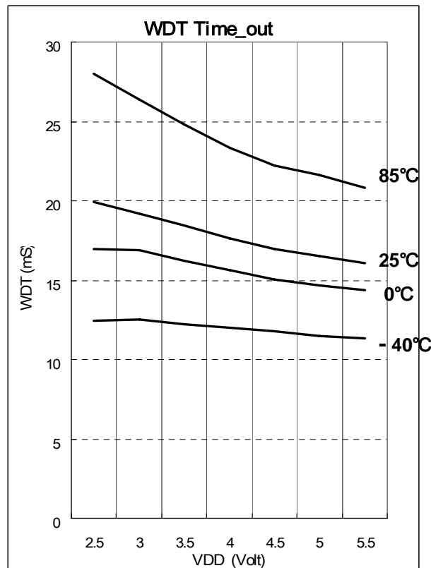
Fig. 7-8 WDT Time out Period vs. VDD, Prescaler Set to 1:1
