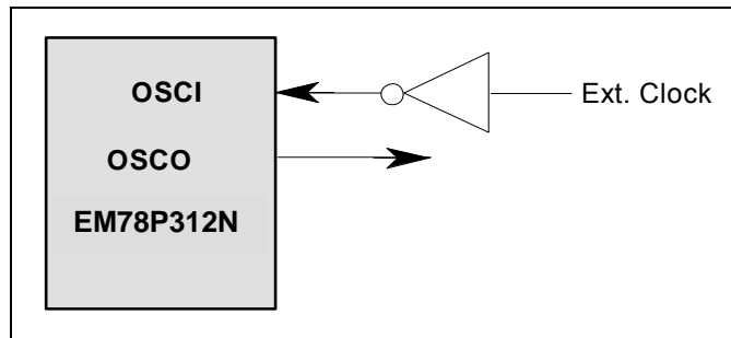
Fig. 5-29 Crystal/Resonator Circuit
