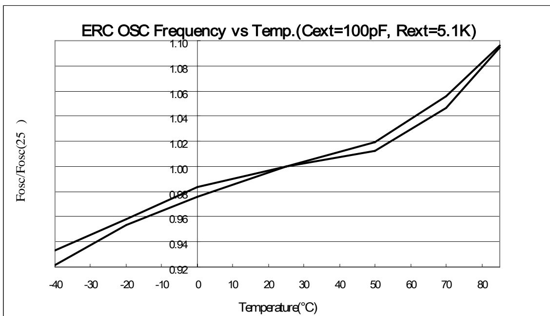
Fig. 7-10 Typical RC OSC Frequency vs. Temperature (R and C are Ideal Components)
