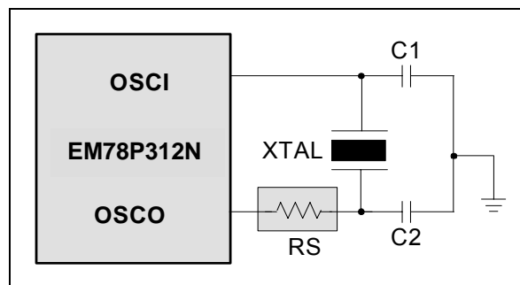
Fig. 5-30 Crystal/Resonator Circuit
