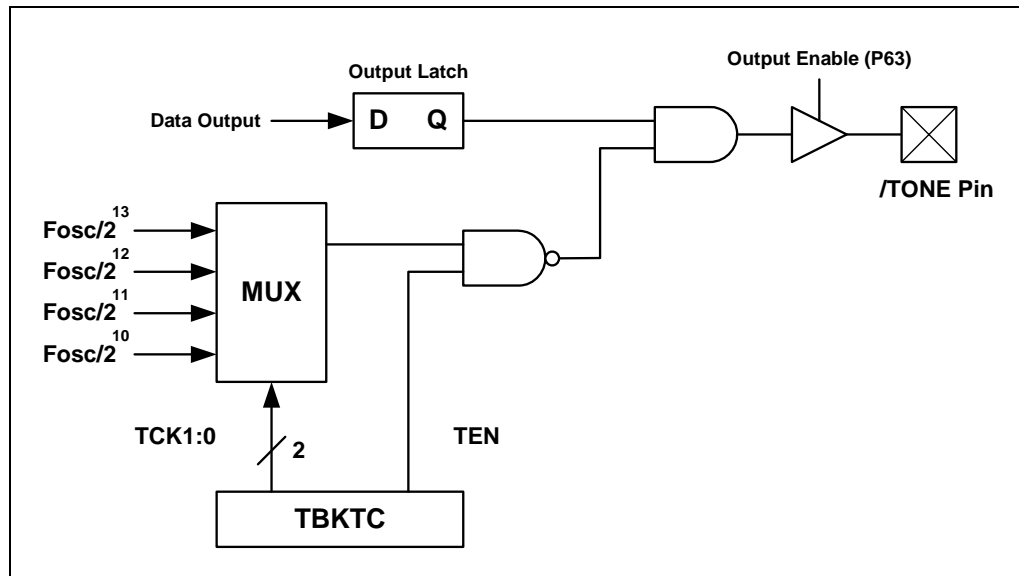
Fig. 5-6 Tone Output Pin Configuration
