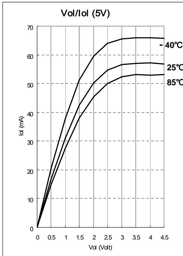
Fig. 7-4 Port 6, Port 7 and Port 8 Vol vs. Iol, VDD=5V
