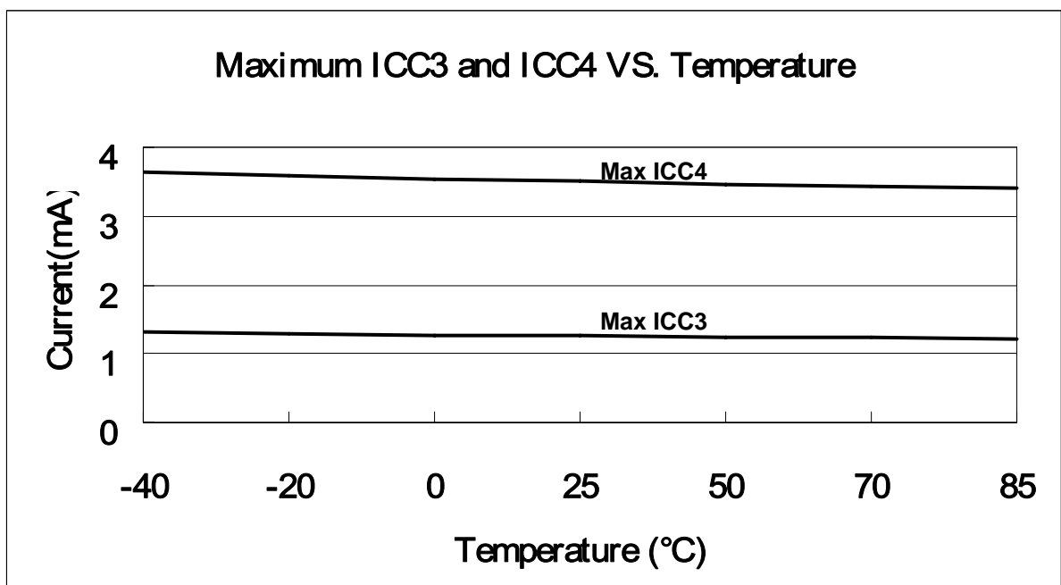
Fig. 7-12 Maximum Operating Current (ICC3 and ICC4) vs. Temperature, VDD=5V
