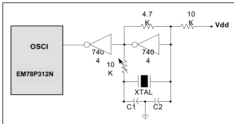
Fig. 5-32 Crystal/Resonator-Parallel Mode Circuit
