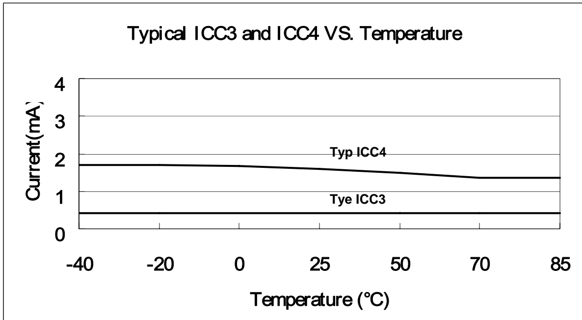
Fig. 7-13 Typical Operating Current (ICC3 and ICC4) vs. Temperature, VDD=3V
