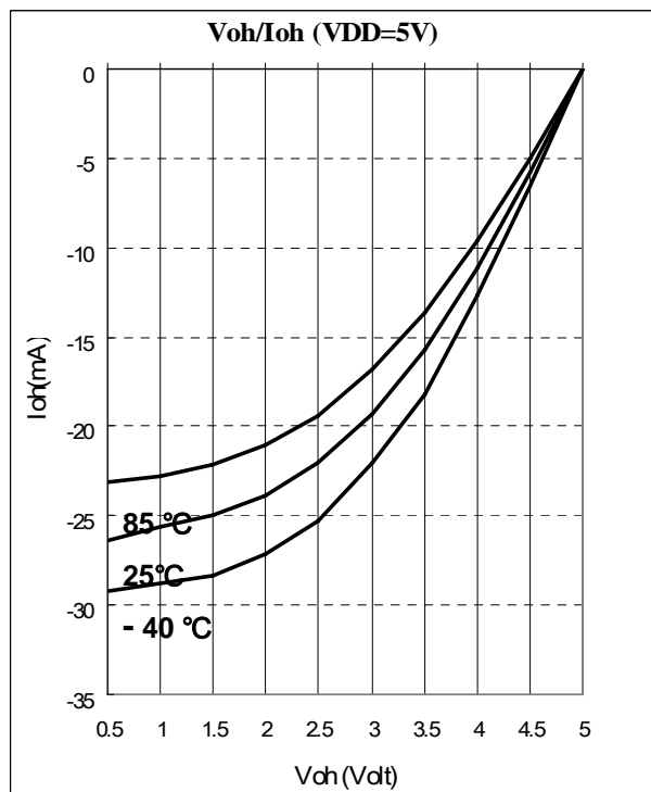
Fig. 7-2 Port 6, Port 7, Port 8 and Port 9 Voh vs. Ioh, VDD=5V
