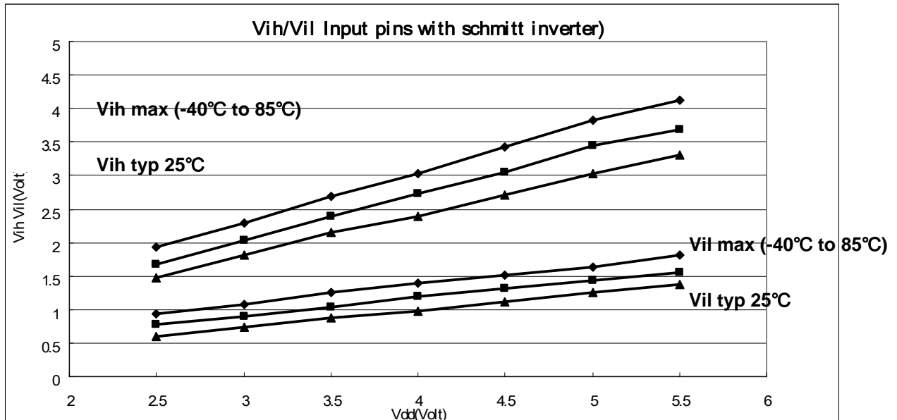
Fig. 7-1 Vih, Vil of P60~P67, P70~P73, P80~P81, P90~P97 vs. VDD
