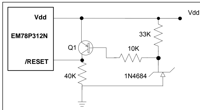
Fig. 5-35 Residue Voltage Protection Circuit 1
