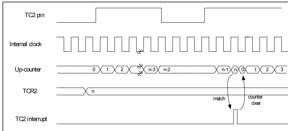
Fig. 5-21 Window Mode Timing Chart
