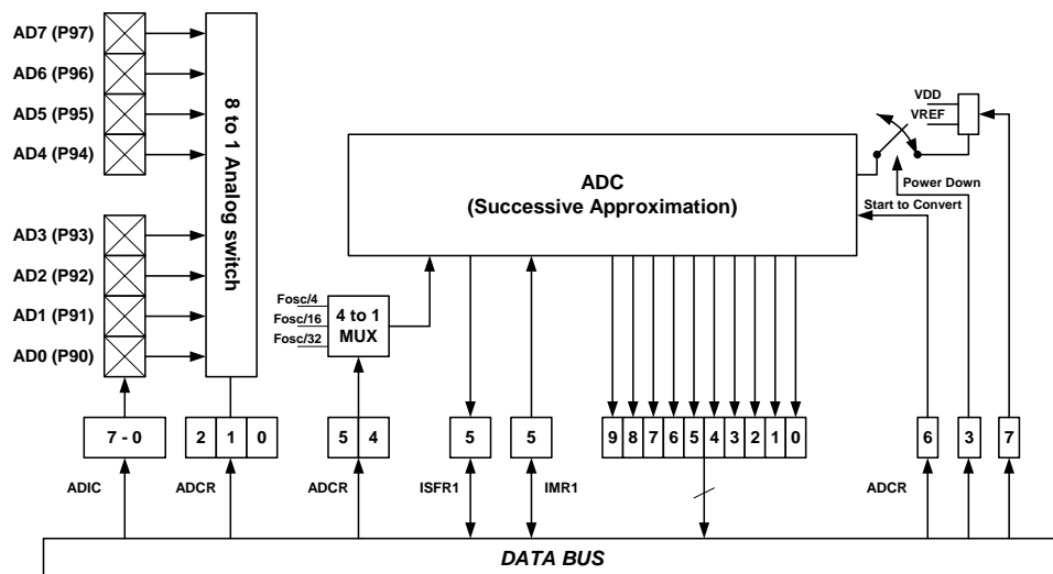
Fig. 5-5 AD Converter
