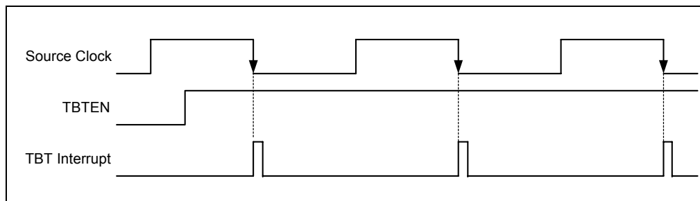
Fig. 5-9 Time Base Timer Timing Chart
