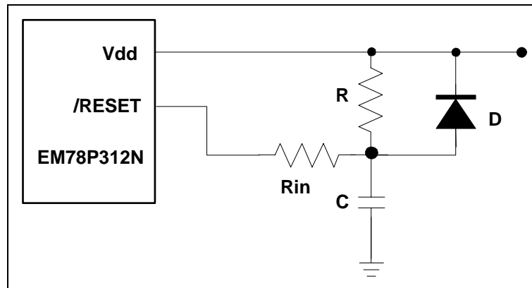
Fig. 5-34 External Power-Up Reset Circuit
