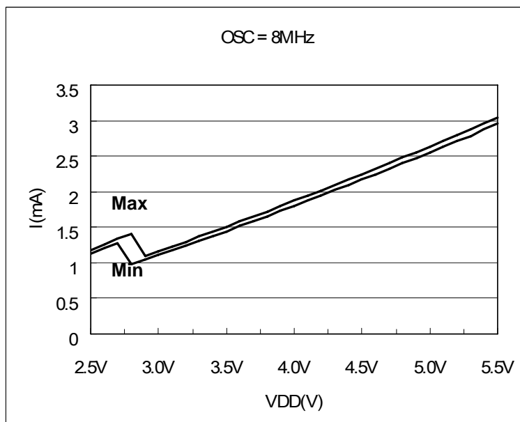
Fig. 7-17 V-I Curve in Operating Mode, Operating Frequency is 8M Hz
