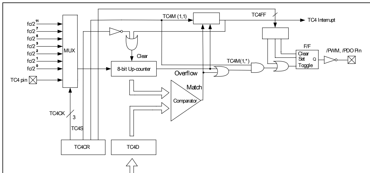
Fig. 5-24 Timer/Counter 4 Configuration
