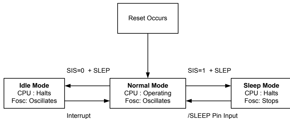
Fig. 5-4 Operation Mode and Switching
