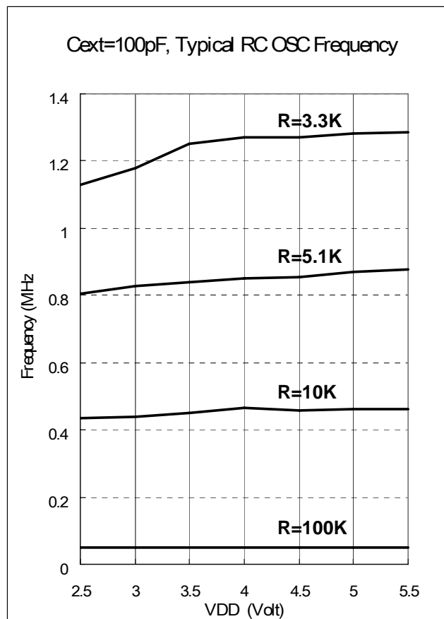
Fig. 7-9 Typical RC OSC Frequency vs. VDD (Cext=100pF, Temperature at 25°C)
