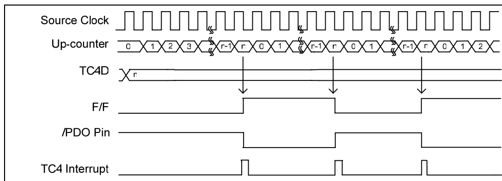
Fig. 5-25 Timing Chart for PDO Mode
