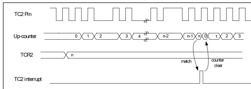
Fig. 5-20 Counter Mode Timing Chart (TC2ES = 1)
