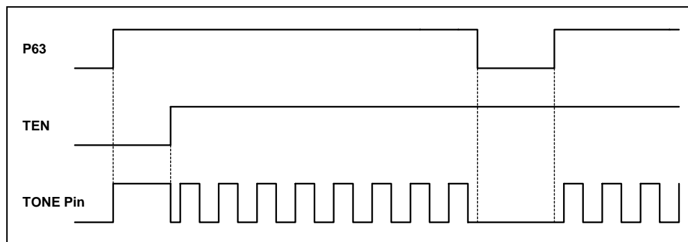
Fig. 5-7 Tone Output Pin Timing Chart
