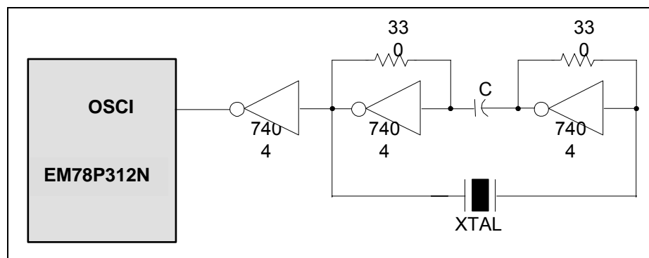
Fig. 5-31 Crystal/Resonator-Series Mode Circuit
