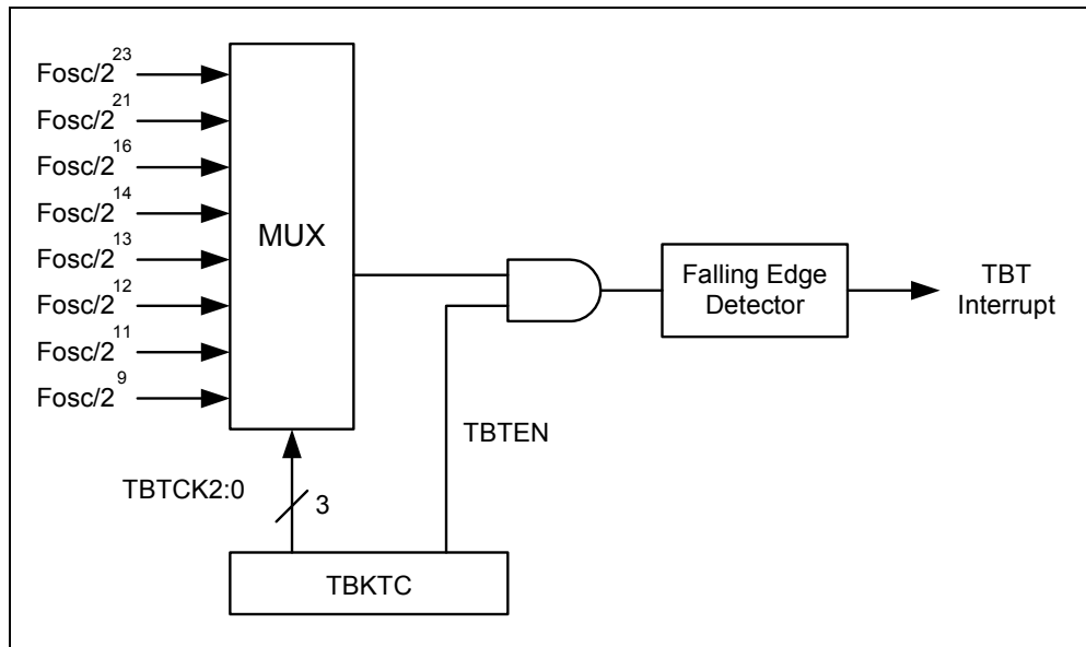
Fig. 5-8 TBT Configuration
