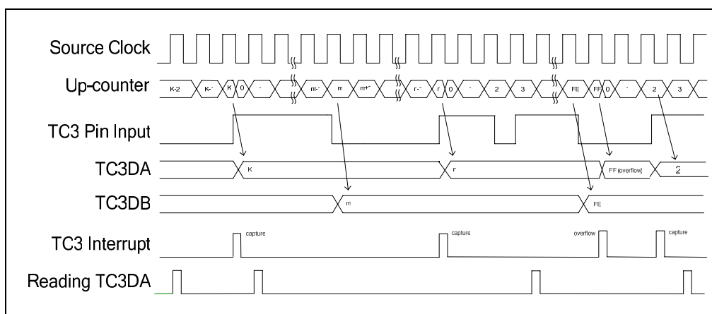
Fig. 5-23 Timing Chart of Capture Mode
