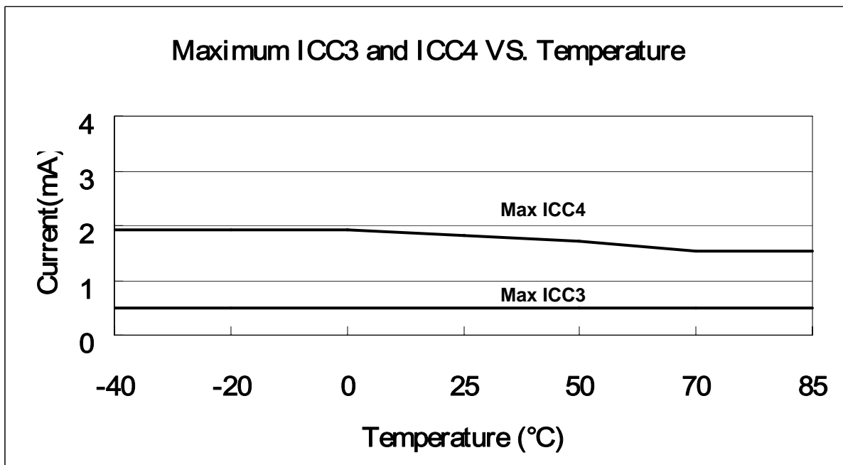
Fig. 7-14 Typical Operating Current (ICC3 and ICC4) vs. Temperature, VDD=3V
