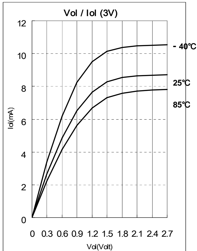
Fig. 7-7 Port 9 Vol vs. Iol, VDD=3V
