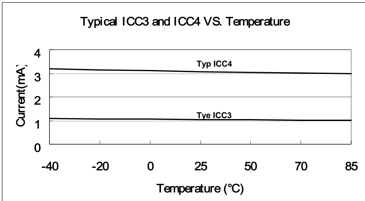
Fig. 7-11 Typical Operating Current (ICC3 and ICC4) vs. Temperature, VDD=5V
