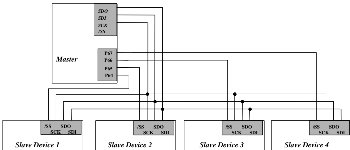
Fig. 5-17 The SPI Configuration Example of Single-Master and Multi-Slaves
