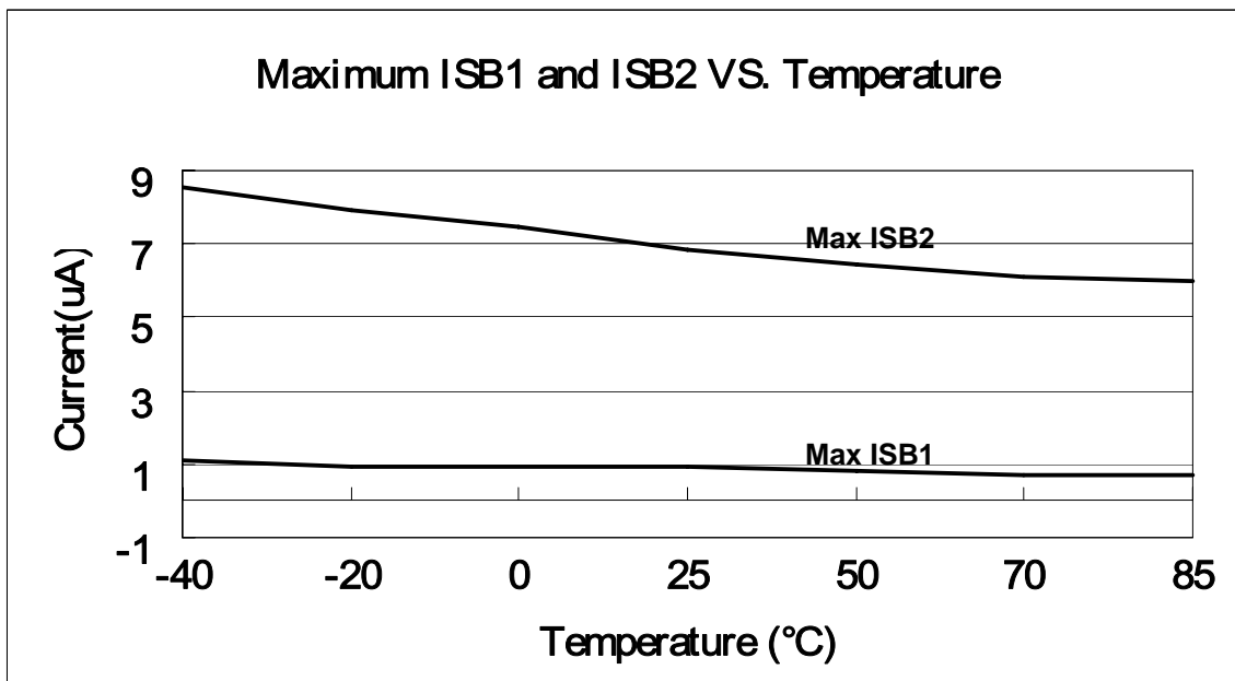
Fig. 7-16 Maximum Standby Current (ISB1 and ISB2) vs. Temperature
