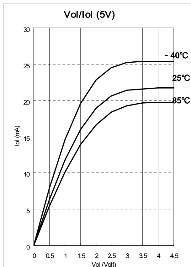
Fig. 7-6 Port 9 Vol vs. Iol, VDD=5V
