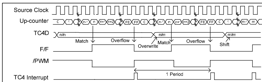
Fig. 5-26 Timing Chart for PWM Mode
