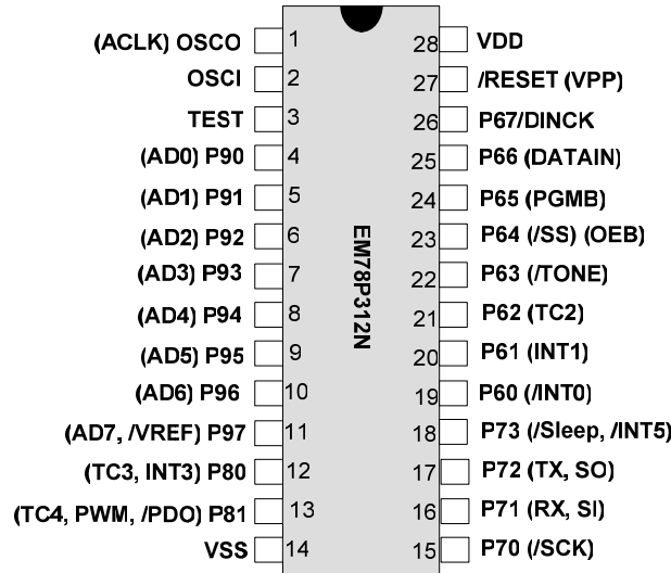
Fig. 3 EM78P312N Pin Assignment
