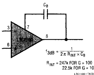
Figure 2. Overcompensation to Reduce System Bandwidth
