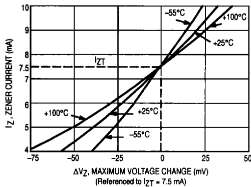
Figure 2. 1N821 Series
