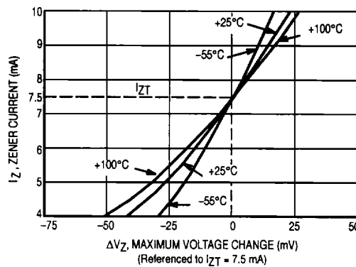
Figure 3. 1N821A Series
