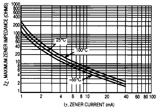
Figure 5. 1N821A Series
