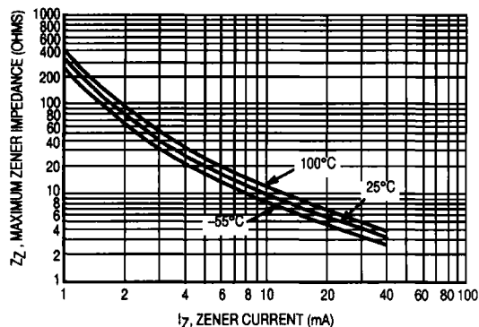
Figure 4. 1N821 Series
