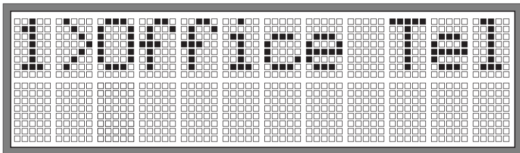
Figure 42 Example of Blink Cursor (LC = 1; B = 1)
