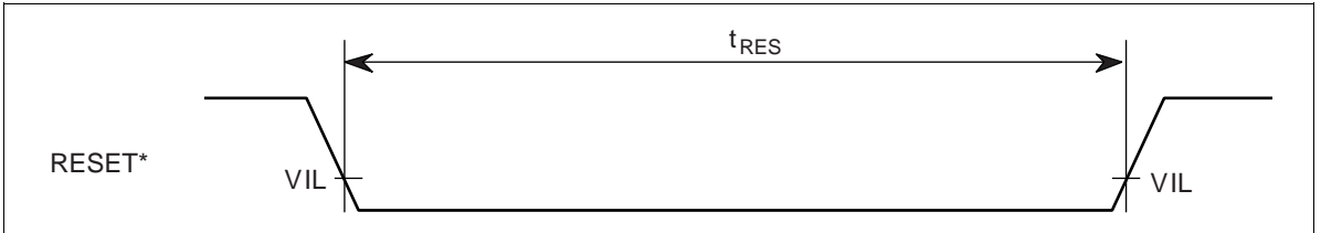
Figure 55 Reset Timing
