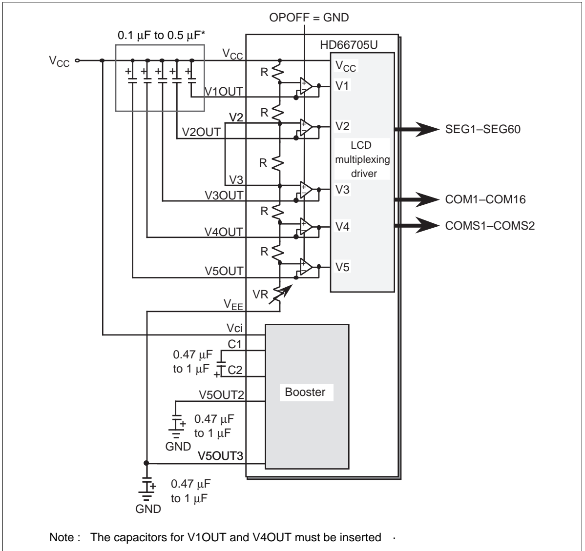
Figure 33 Operational Amplifier Output Stabilization Circuit Example
