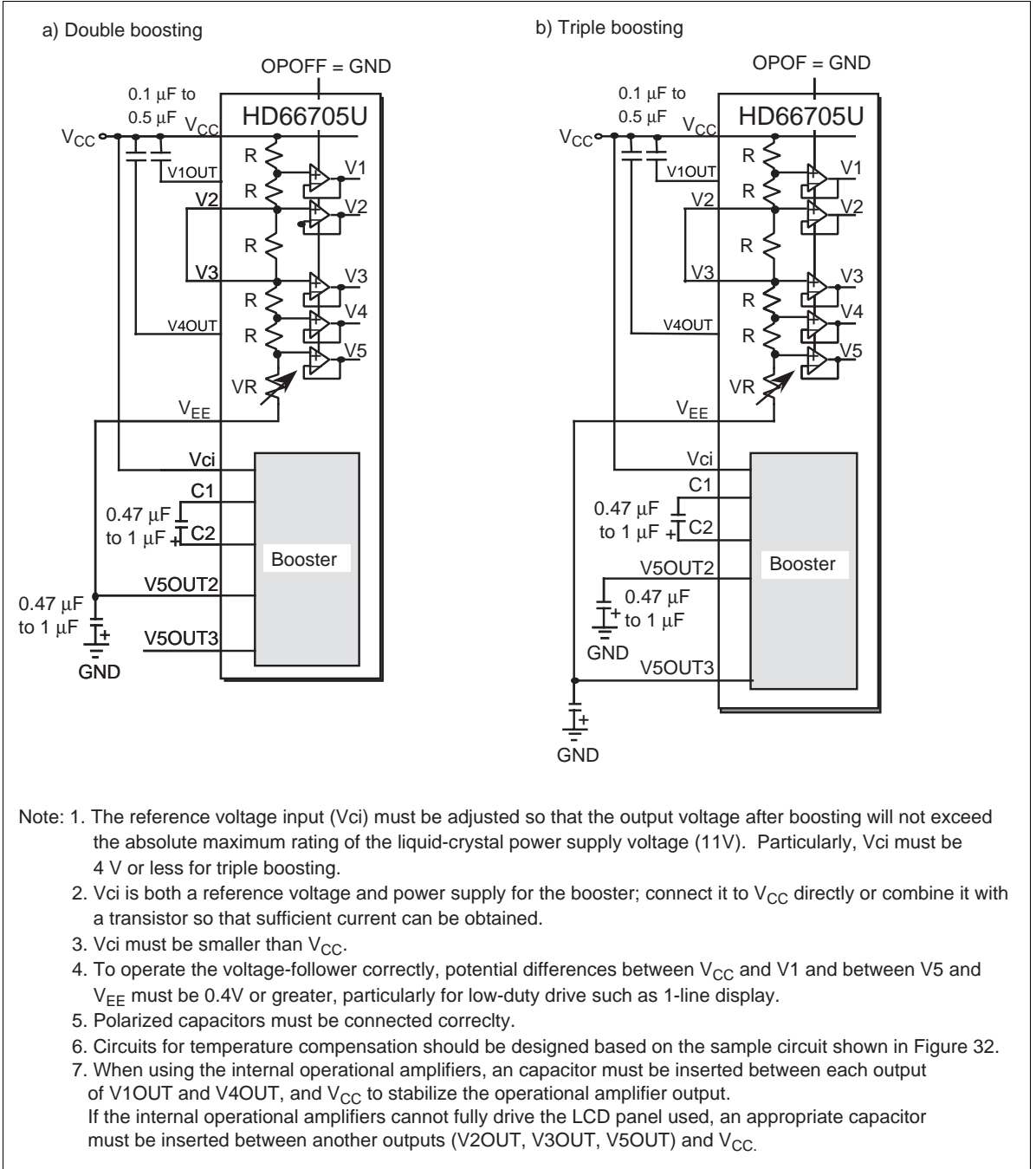
Figure 31 Internal Power Supply Circuit Example for LCD Drive Voltage Generation
