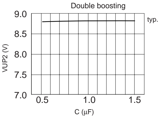
Figure 50 Booster (cont)
