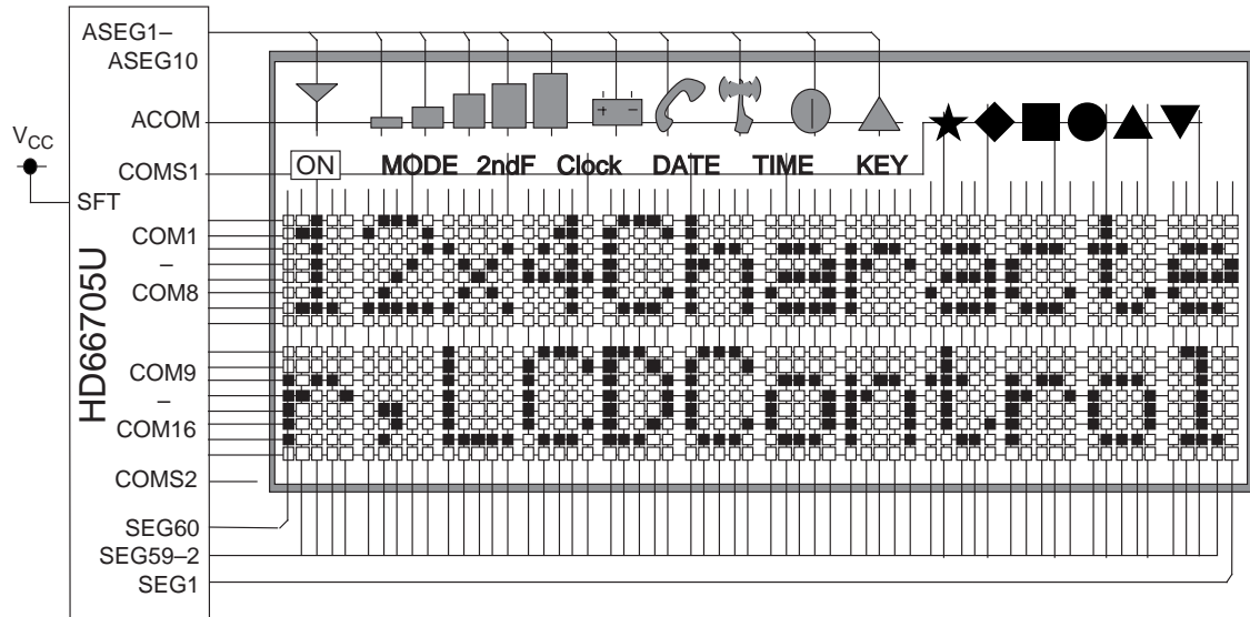
b) 12-character x 2-line display (SEG line below the panel : SFT = V CC )
