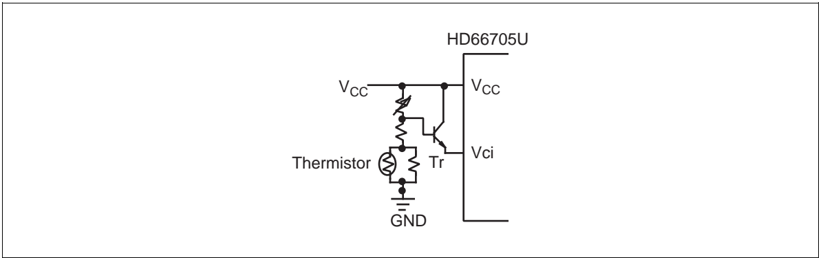
Figure 32 Temperature Compensation Circuit Example
