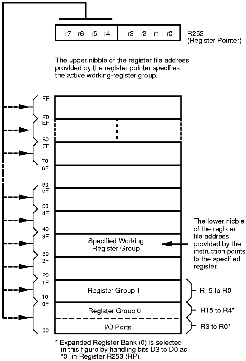
Figure 25. Register Pointer
