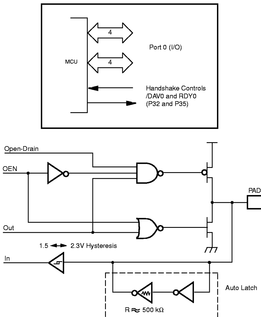
Figure 18. Port 0 Configuration
