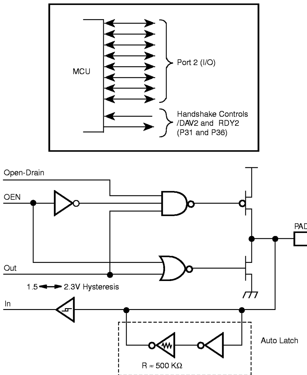
Figure 20. Port 2 Configuration
