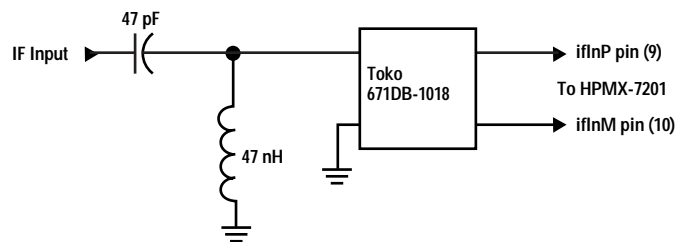
Figure 32. Test Circuit for Single-ended 50Ω IF Operation.
