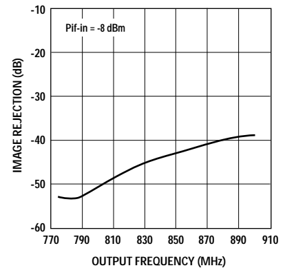
Figure 18. AMPS Upconverter Image Rejection vs. Output Frequency.
