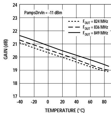
Figure 20. AMPS Driver Gain vs. Temperature and Frequency.
