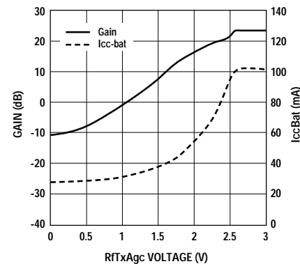
Figure 35. HPMX-7201 RF VGA Gain and Supply Current Consumption vs. RfTxAgc Voltage.
