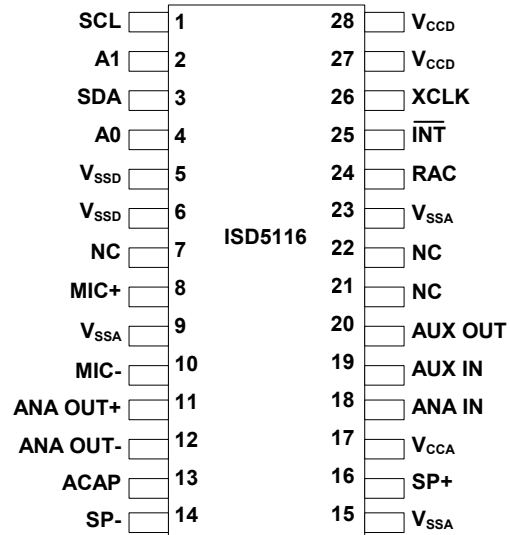
PDIP
