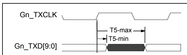
Figure 25 - AC Characteristics – Ten Bit Interface (RX)
