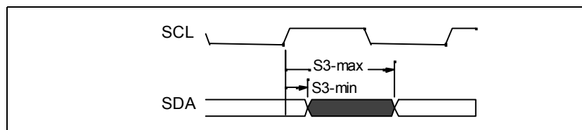
Figure 33 - I 2 C Output Delay Timing
