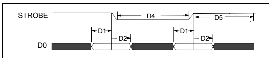
Figure 34 - Serial Interface Setup Timing
