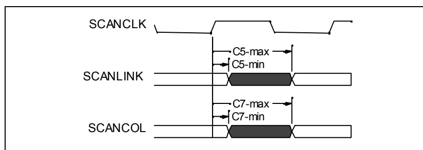
Figure 28 - SCANLINK, SCANCOL Output Delay Timing
