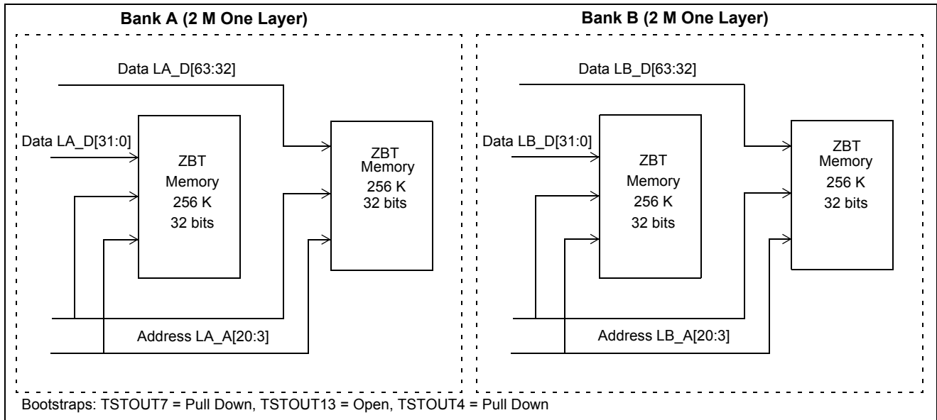
Figure 13 - ZBT Memory Configuration For 2 M/bank, 1 Layer
