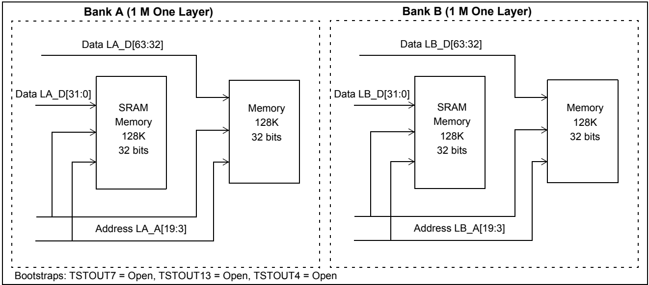
Figure 9 - Memory Configuration For 1 M/bank, 1 Layer
