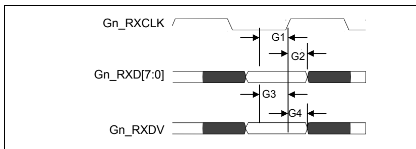
Figure 24 - AC Characteristics – Gigabit Media Independent Interface
