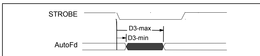
Figure 35 - Serial Interface Output Delay Timing
