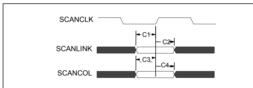
Figure 29 - SCANLINK, SCANCOL Setup Timing
