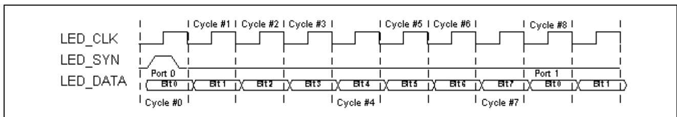
Figure 5 - Timing Diagram of LED Interface
