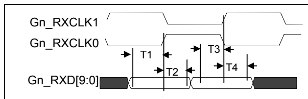
Figure 26 - AC Characteristics –Ten Bit Interface (TX)
