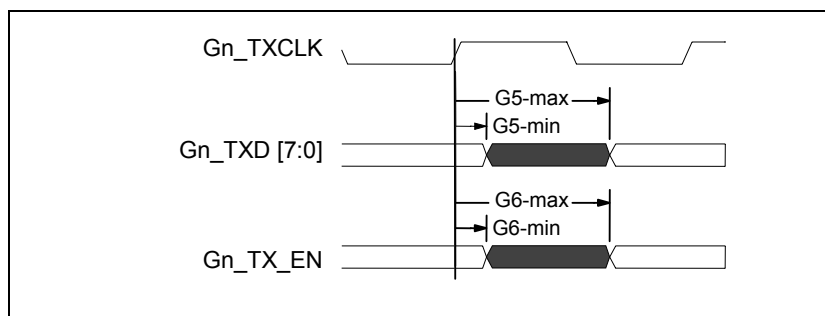
Figure 23 - AC Characteristics- Gigabit Media Independent Interface
