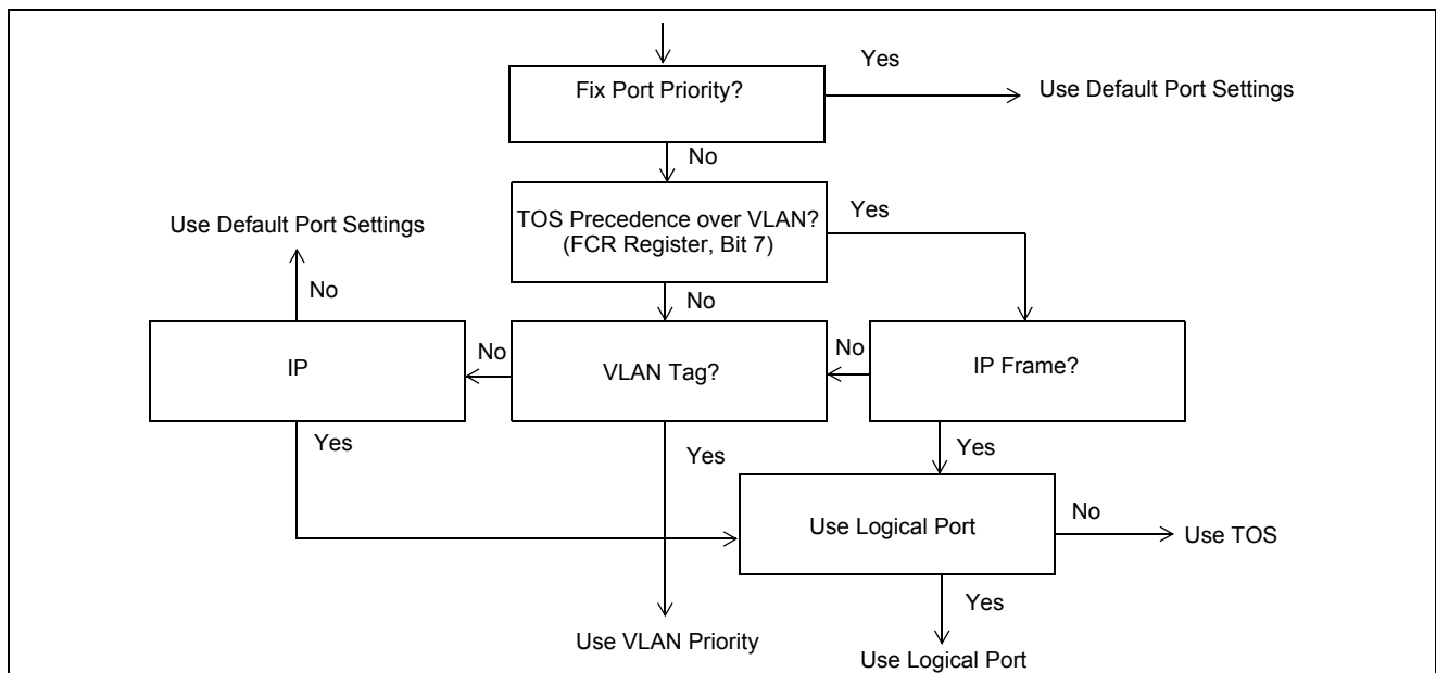
Figure 14 - Priority Classification Rule
