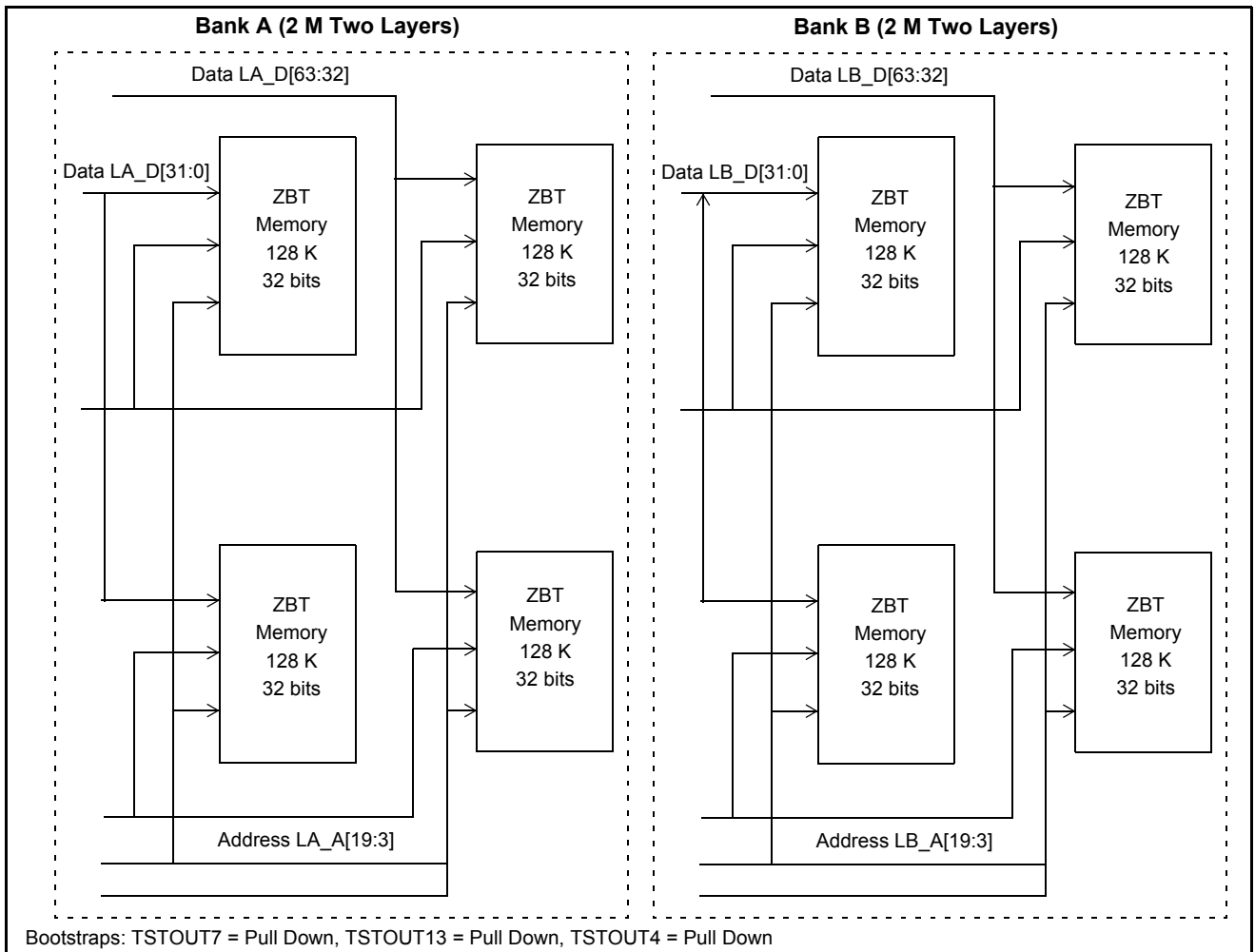
Figure 12 - ZBT Memory Configuration For 2 M/bank, 2 Layers
