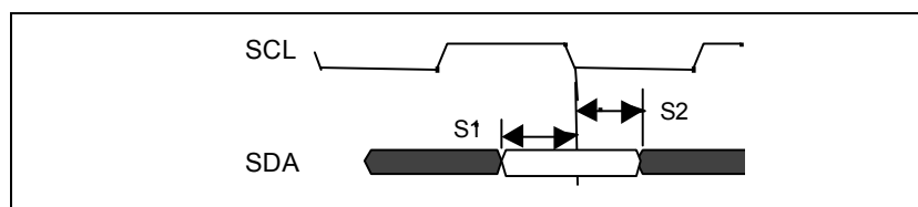
Figure 32 - I 2 C Input Setup Timing
