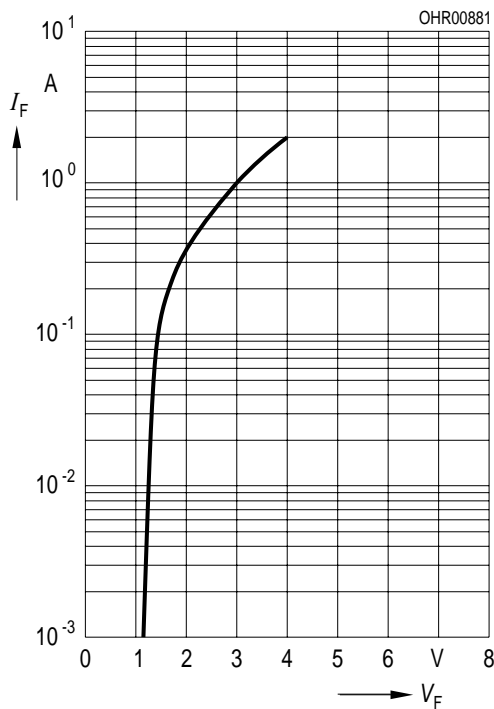
Forward Current 1) I_F = f(V_F) , Single pulse, t_p = 20\ ms , T_A = 25\text{ °C}
