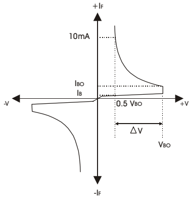
DIAGRAM 1: Current-voltage characteristics
