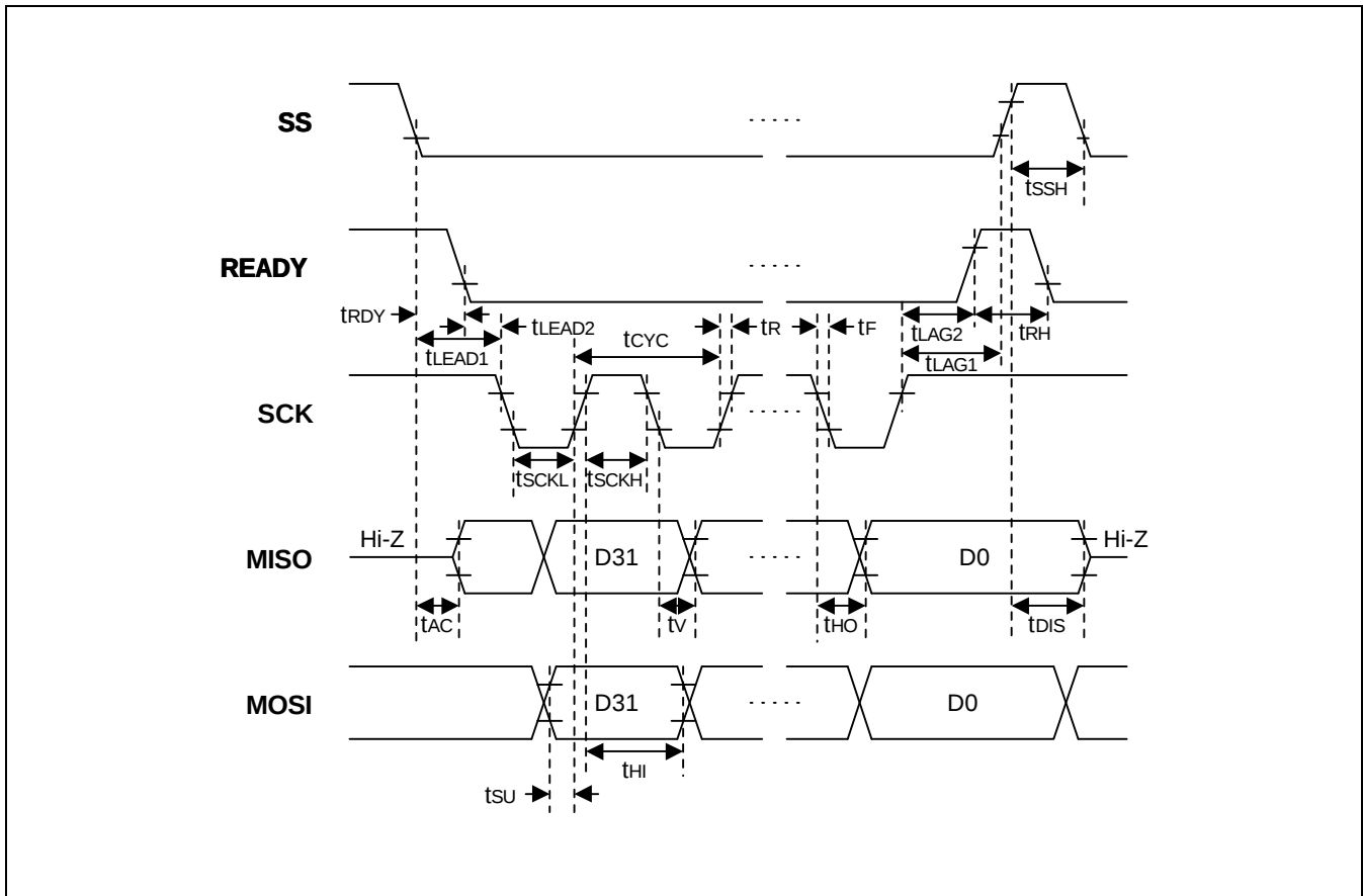
Figure 15: SPI Timing
