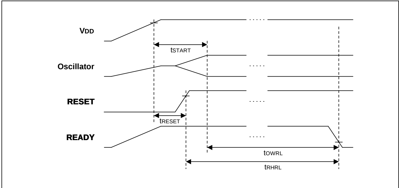
Figure 16: Start-up Timing
