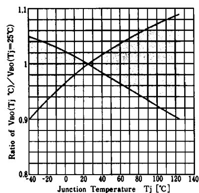
Breakover Voltage VS. T_J
