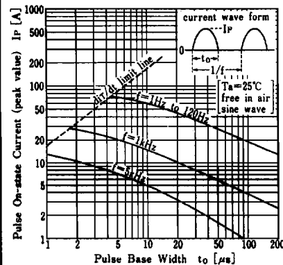
Pulse On-state Current Rating (I_TRM)
