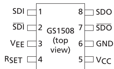
Figure 1-1: Pin Assignment
