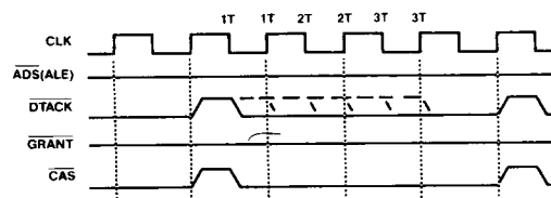
Figure 19. DTACK While Bursting 68040 in Burst Mode
