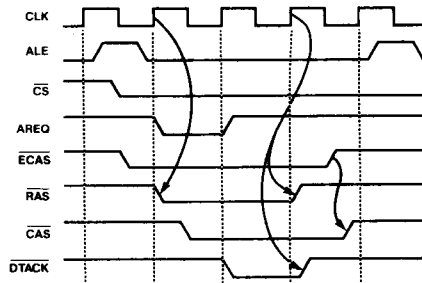
Figure 6. Single Access Mode with Synchronous Access Start and Extended CAS
