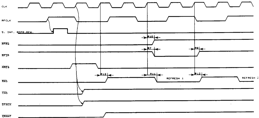
Figure 48. REFRESH with Extend Refresh
