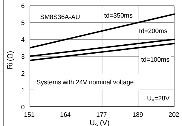
Fig.12 ISO-16750-2 TYPE A
