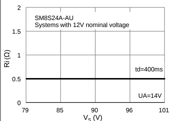
Fig.11 ISO-16750-2 TYPE A
