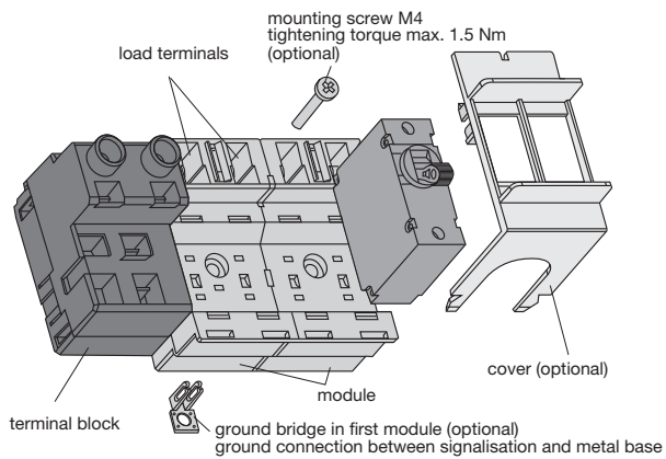
Distribution rail, shown with power supply left-side X8340-S02L-...
