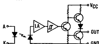
OPB10512/OPB10532 (Totem-Pole Output) Inverter
