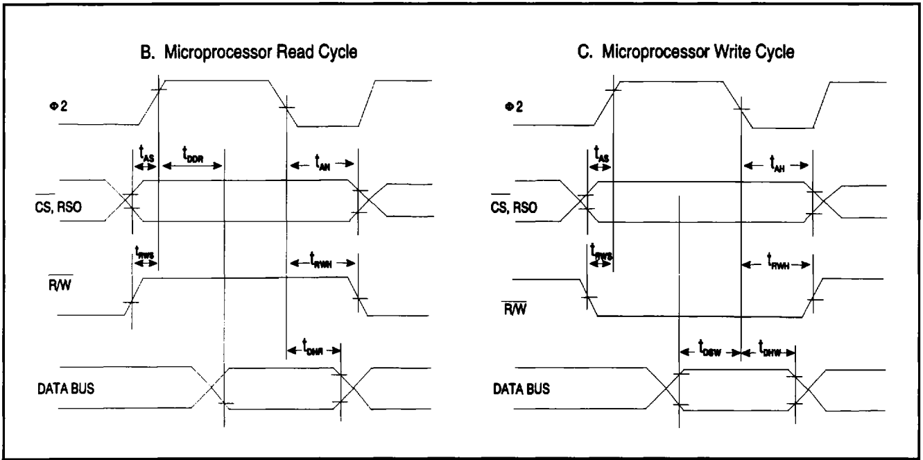
Figure 11 Timing Diagrams (concluded)
