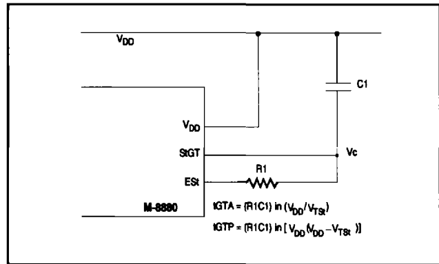
Figure 5 Basic Steering Circuit
