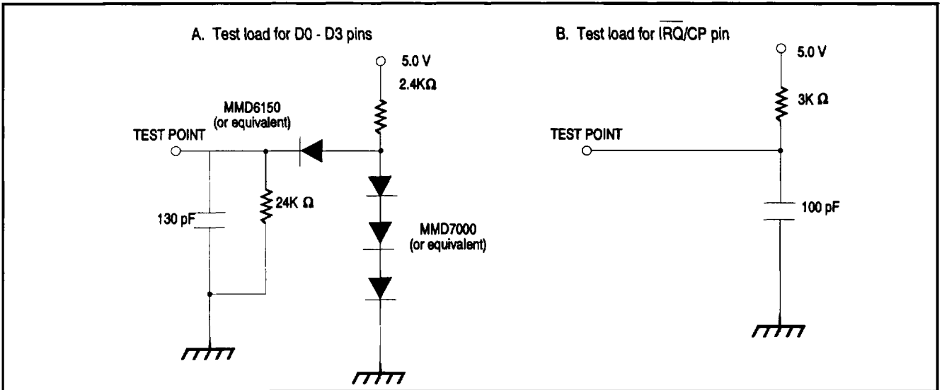
Figure 12 Test Loads
