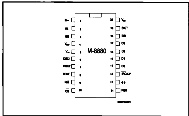
Figure 1 Pin Diagram
