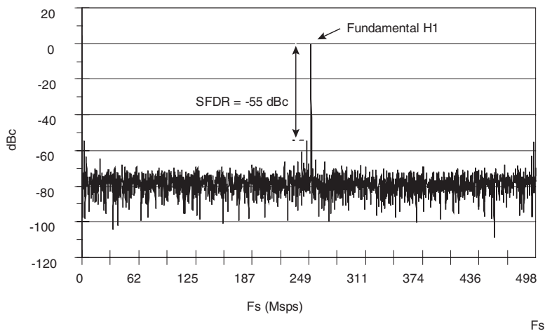
Figure 9-16. F_s = 500 Msp and F_{in} = 250 MHz (Interleaving Mode F_{int} = 1 Gsp 1:1 DMUX, F_iSDA = -35 ps, ISA = 0 ps)
