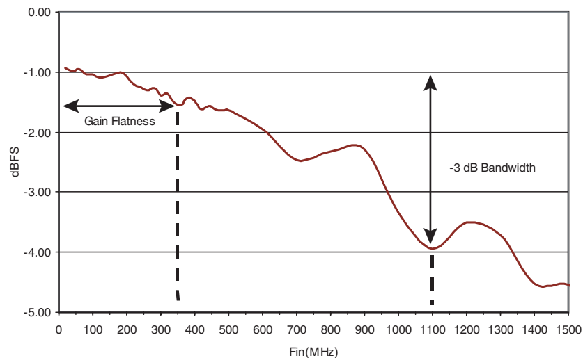
Figure 9-1. Full Power Input Bandwidth
