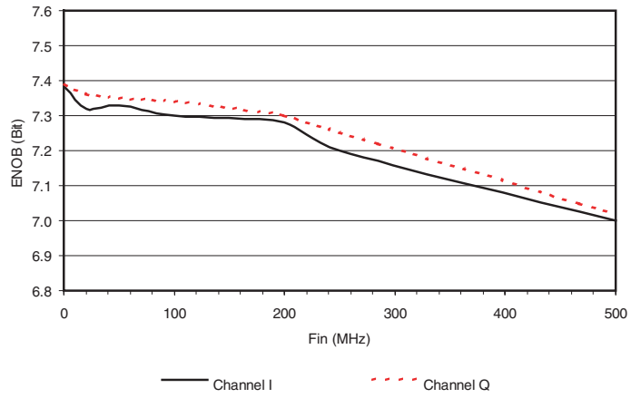
Figure 9-9. ENOB Versus Input Frequency ( F_s = 500 Msp/s)
