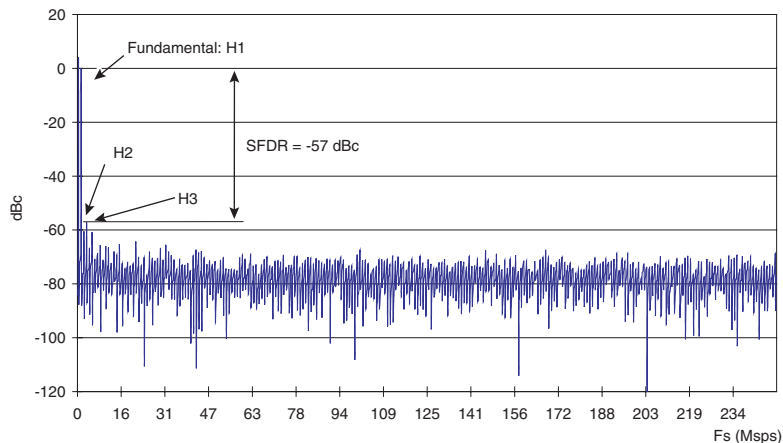
Figure 9-15. F_s = 500 Msp and F_{in} = 500 MHz (1:2 DMUX, F_s/4 DR Type F_iSDA = -35 ps, ISA = 0 ps)
