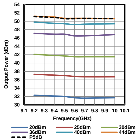
Output Power vs. Frequency V_{DS}=24V , I_{DS(DC)}=5.3A PW=100\mu sec , Duty 10%
