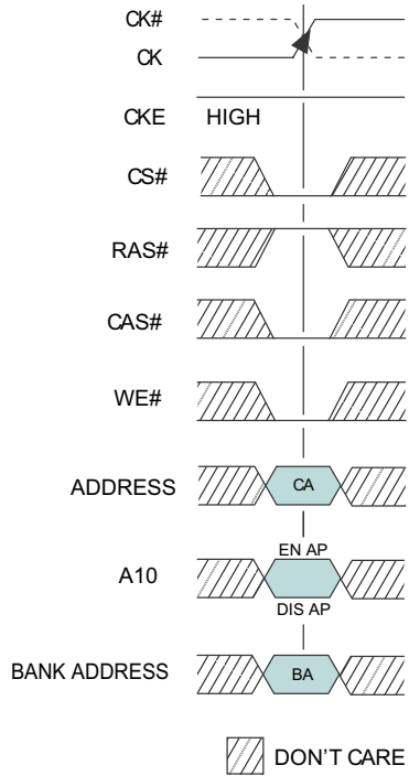
FIGURE 12 – WRITE COMMAND
