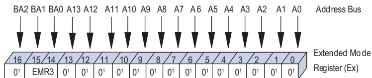
FIGURE 9 – EXTENDED MODE REGISTER 3 (EMR3) DEFINITION
