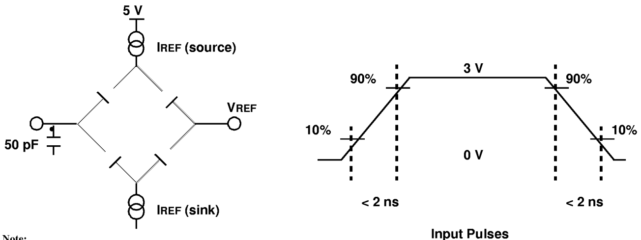
Figure 32b. AC Test Loads and Input Waveforms
