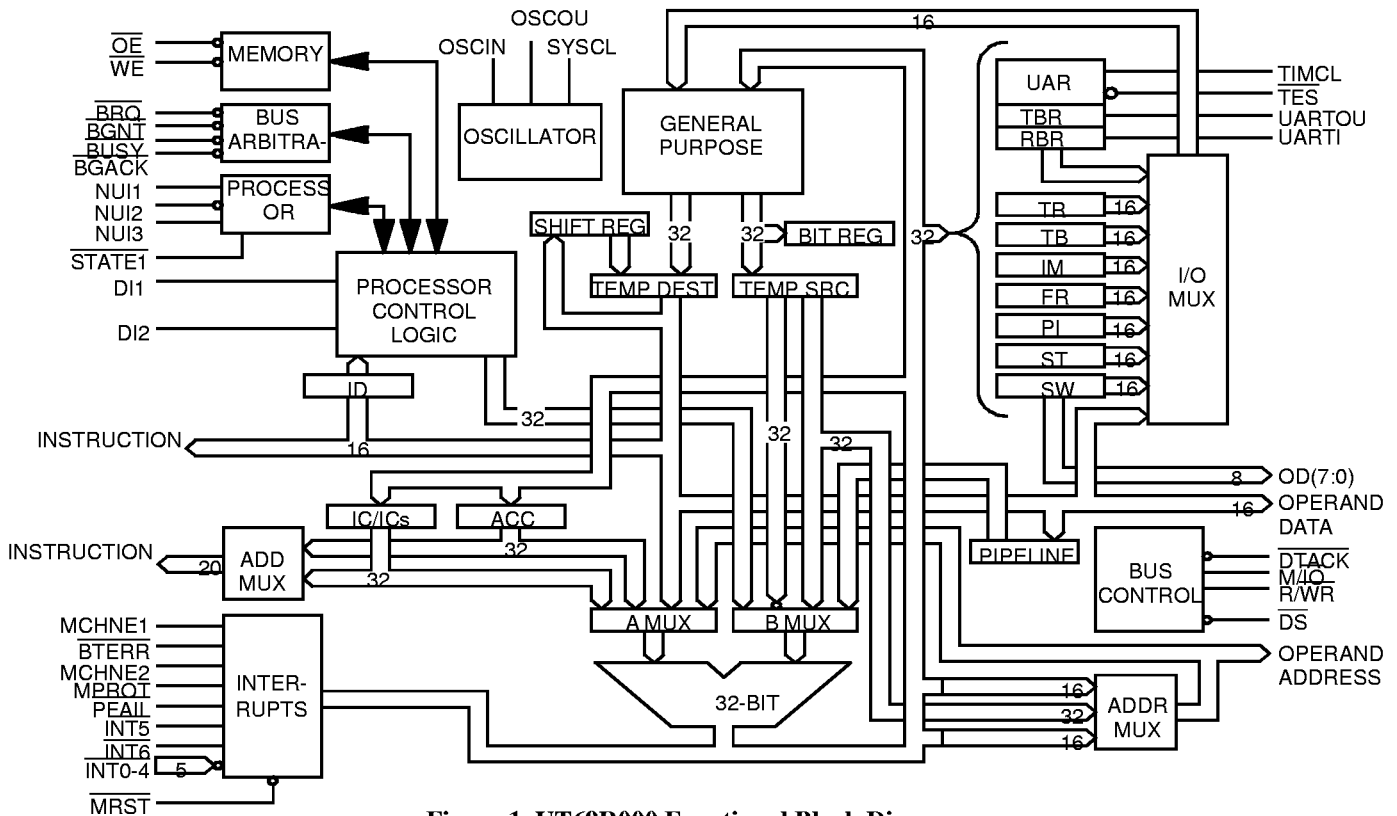
Figure 1. UT69R000 Functional Block Diagram
