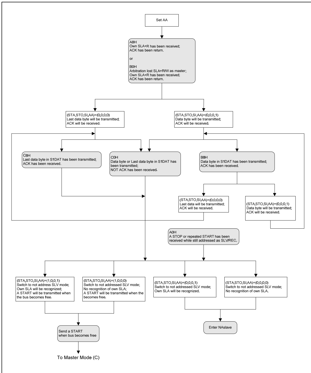
Figure 24-6: Slave Transmitter Mode
