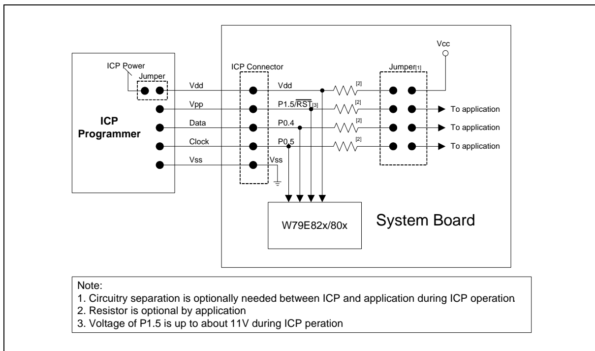
Figure 25-1: Application Circuit of ICP
