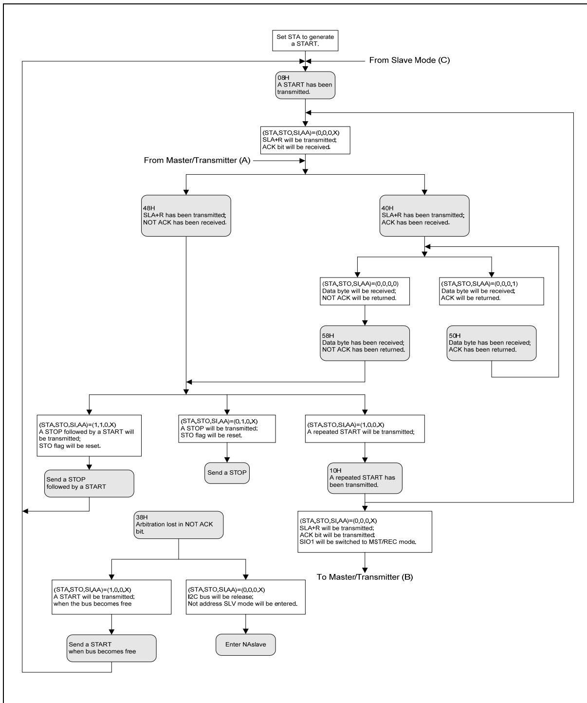
Figure 24-5: Master Receiver Mode
