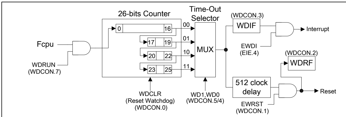
Figure 15-1: Watchdog Timer
