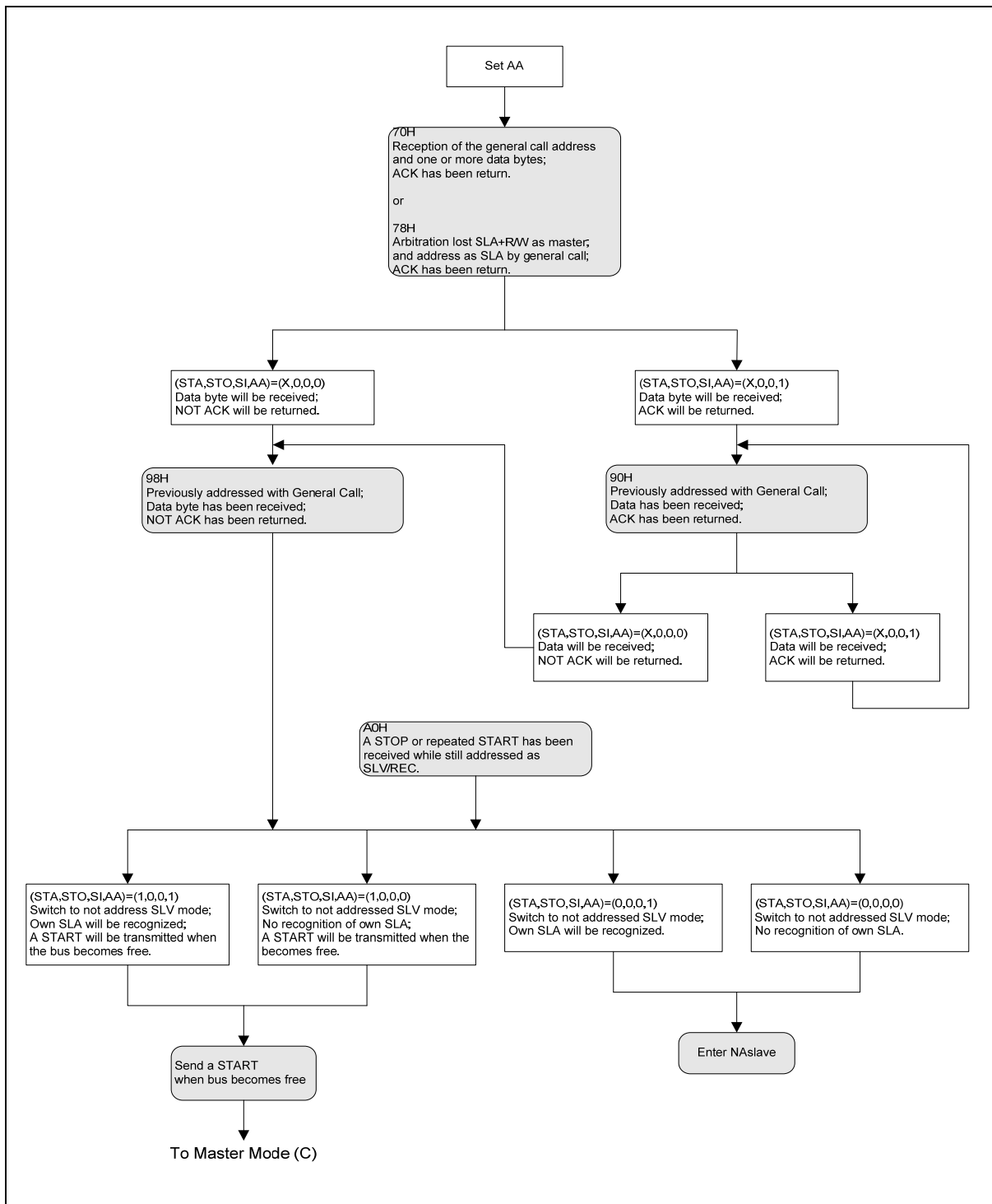
Figure 24-8: GC Mode
