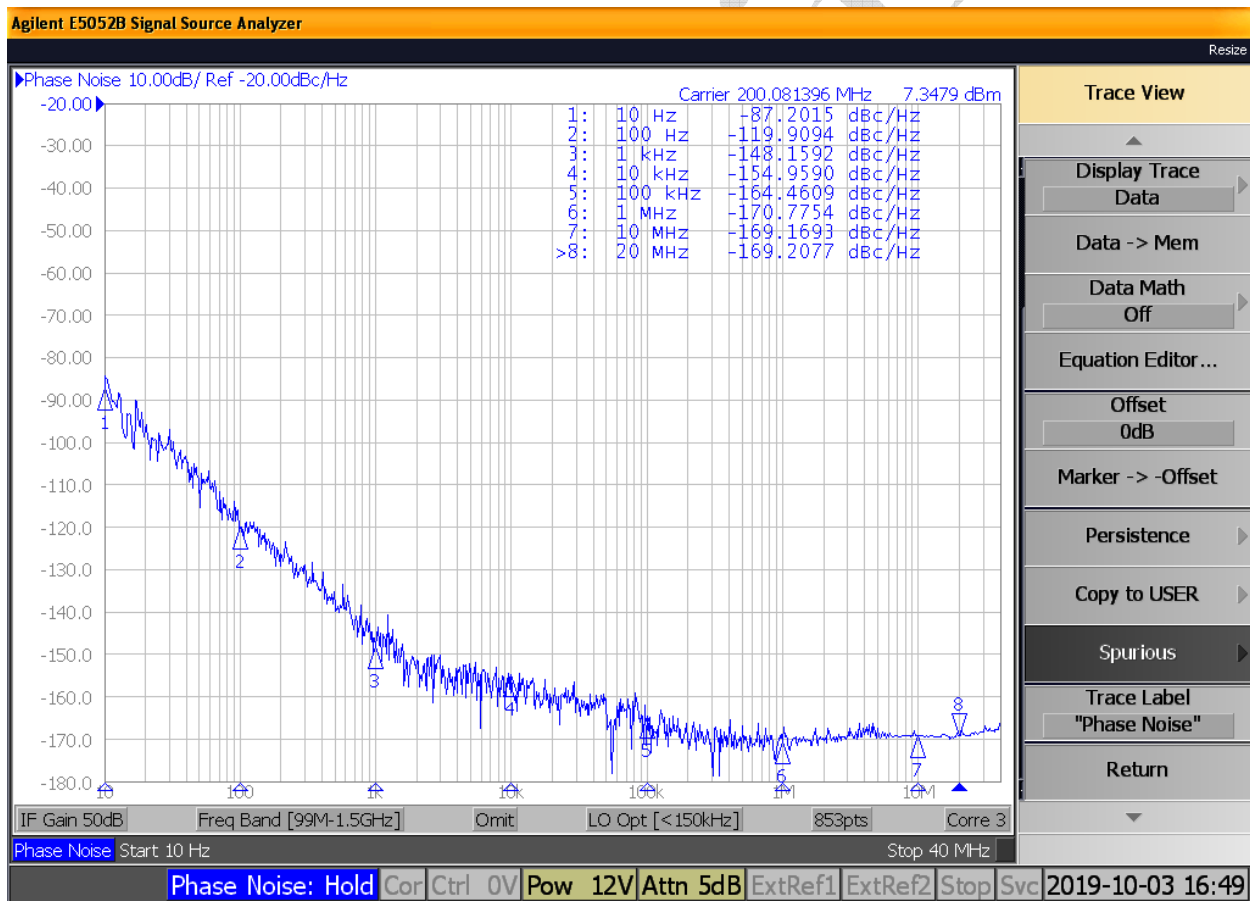
FIGURE 1 – Typical Phase Noise @ 200MHz 12V
