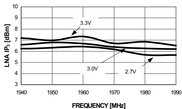
LNA Input IP_3 vs. V_{DD} , RF Input = -30 dBm @ 25°C, V_{DD} = 2.7V, 3.0V, 3.3V
