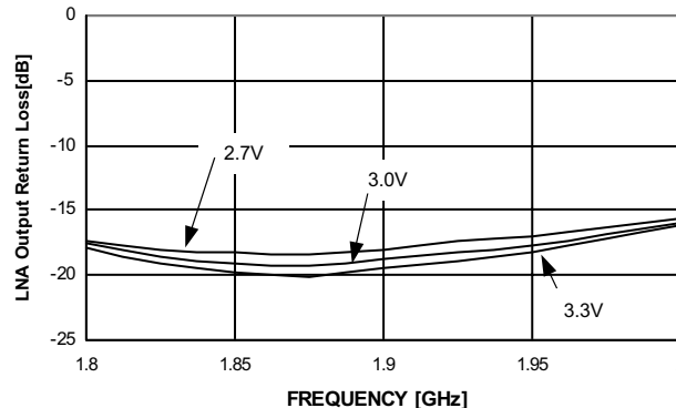
LNA Output Return Loss vs. V_{DD} @ 25°C, V_{DD} = 2.7V, 3.0V, 3.3V
