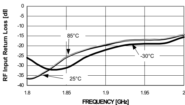
Downconverter RF Input Return Loss vs. Temperature @ 25°C, 85°C, -30°C, V_{DD} = 3.0V, V_{CTRL} = 3.0V
