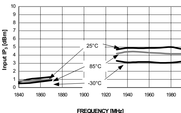
Downconverter Input IP_3 vs. Temperature @ 25°C, 85°C, -30°C, V_{DD} = 3.0V , V_{CTRL} = 3.0V , RF Input = -30 dBm, LO = -10 dBm
