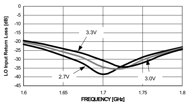
Downconverter LO Input Return Loss vs. V_{DD} Temperature @ 25°C, V_{DD} = 2.7V, 3.0V, 3.3V
