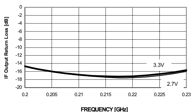
Downconverter IF Output Return Loss vs. V_{DD} Temperature @ 25°C, V_{DD} = 2.7V , 3.0V, 3.3V, V_{CTRL} = 3.0V
