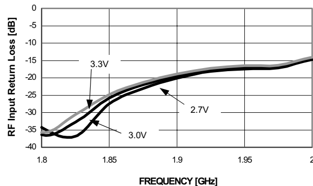
Downconverter RF Input Return Loss vs. V_{DD} @ 25°C, V_{DD} = 3.2V, 3.0V, 3.3V V_{CTRL} = 3.0V
