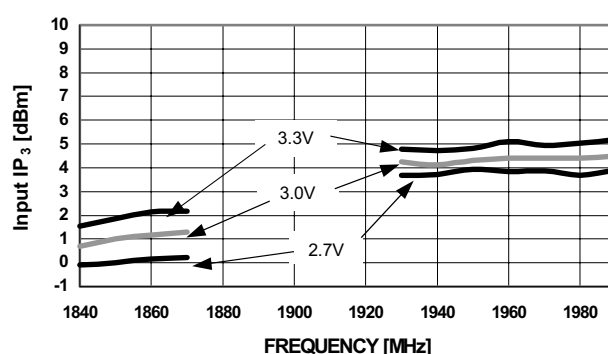
Downconverter Input IP_3 vs. V_{DD} Temperature @ 25°C, V_{DD} = 2.7V , 3.0V, 3.3V, V_{CTRL} = 3.0V , RF Input = -30dBm, LO = -10dBm
