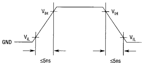
Input Waveforms
