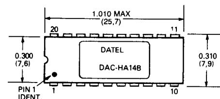
20-PIN DIP CERAMIC PACKAGE
