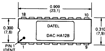
18-PIN DIP CERAMIC PACKAGE
