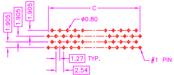
RECOMMEND P.C.B. LAYOUT (50 PINS) BOTTOM VIEW
