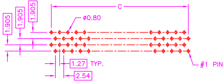
RECOMMEND P.C.B. LAYOUT (68, 80 PINS) BOTTOM VIEW
