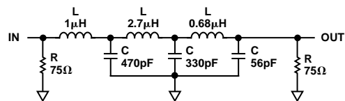
Figure 79. Output Filter
