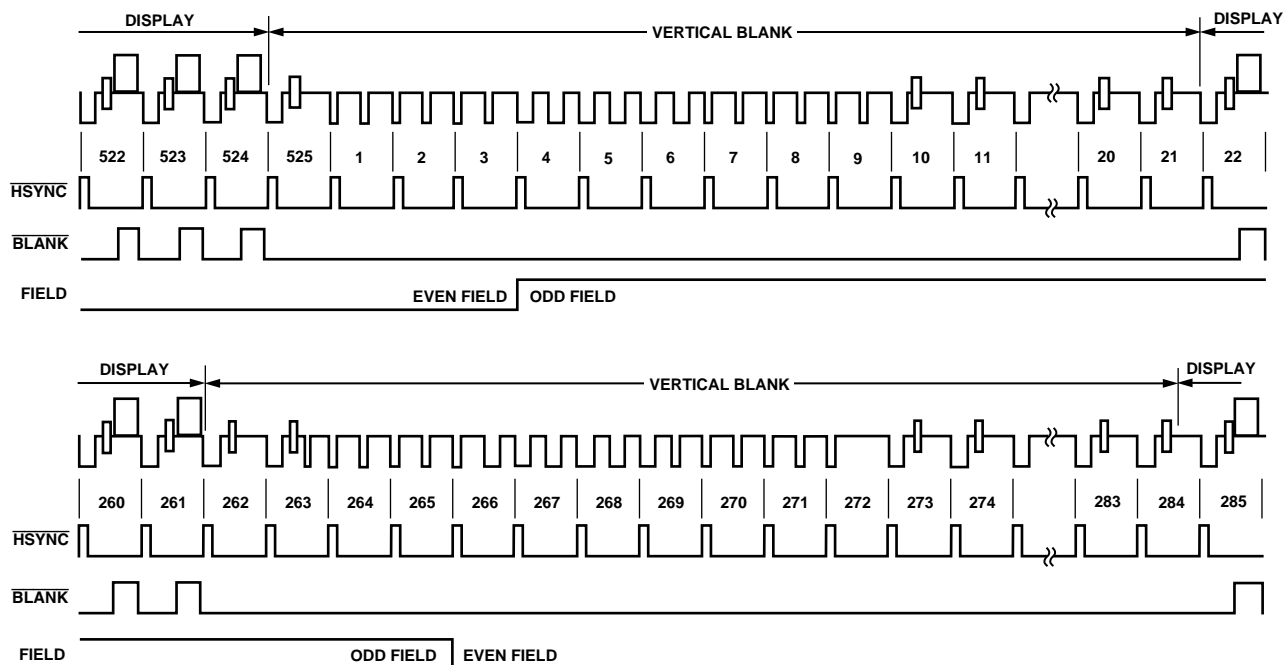
Figure 31. Timing Mode 3 (NTSC)
