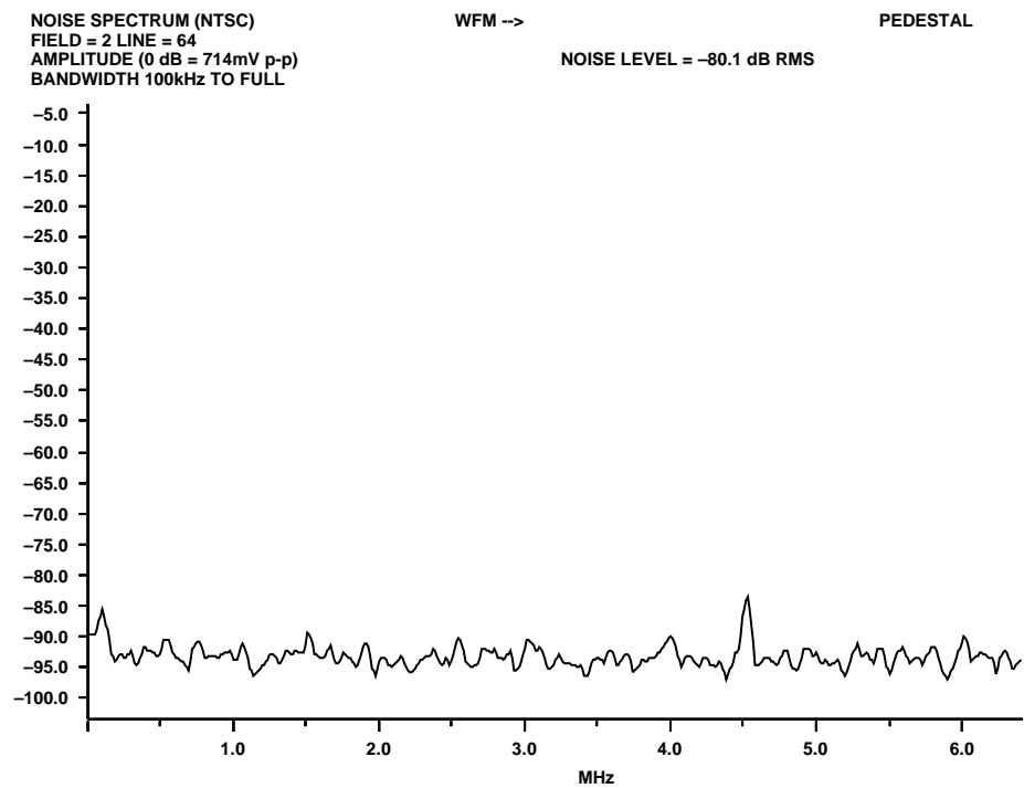
Figure 97. NTSC SNR Pedestal Measurement
