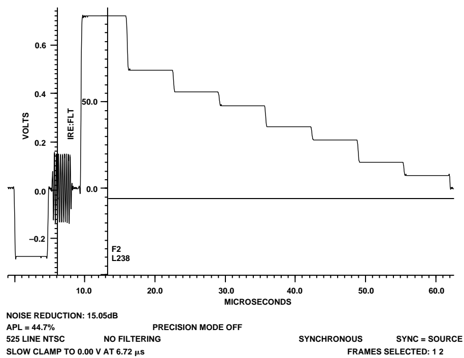
Figure 89. 100%/75% NTSC Color Bars Luminance
