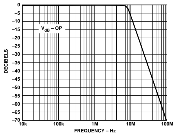
Figure 80. Output Filter Plot
