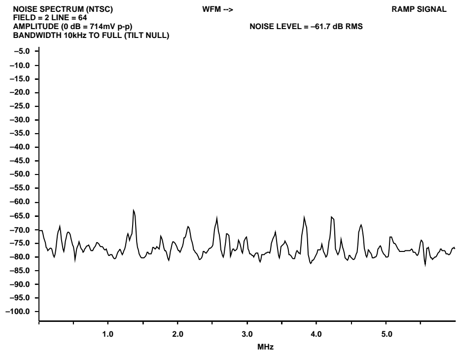
Figure 98. NTSC SNR Ramp Measurement
