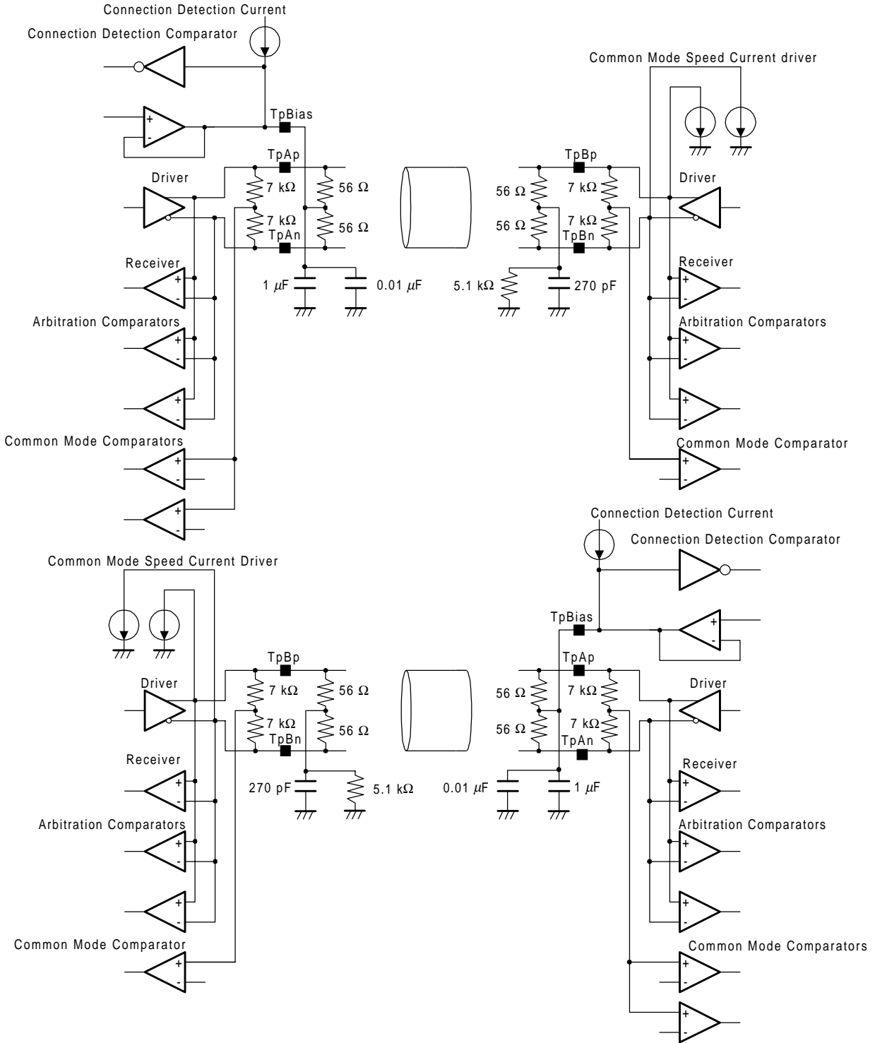
Figure 3-4. Cable Interface
