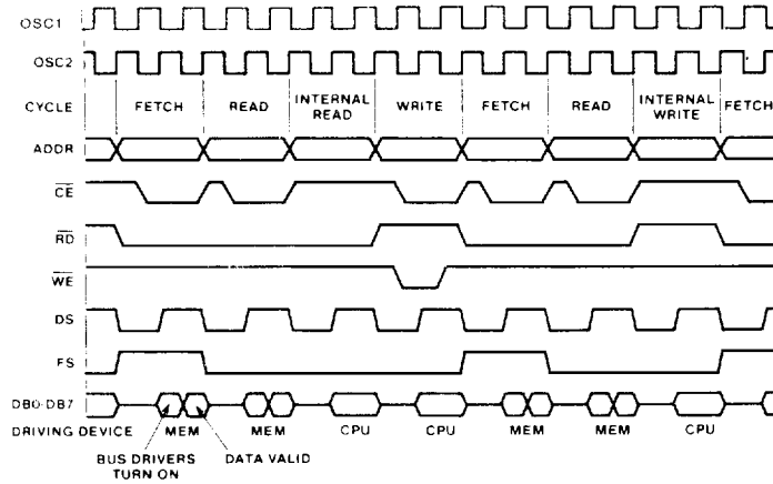
FIGURE 4. CDP68EM05D2N EMULATOR TYPICAL CYCLE TIMING.
