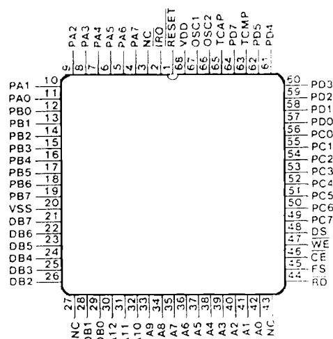
CDP68EM05D2N 68 LEAD PLASTIC CHIP CARRIER
