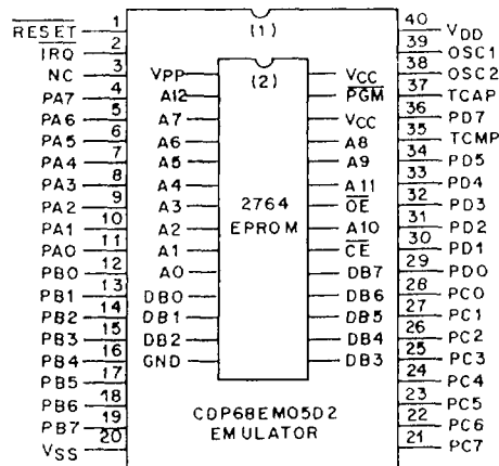
CDP68EM05D2 40 LEAD PIGGYBACK PACKAGE
