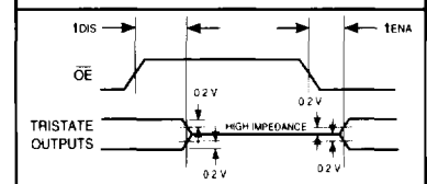
FIGURE 2. THRESHOLD LEVELS
