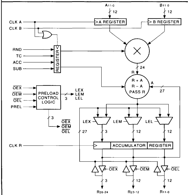
LMA1009/2009 BLOCK DIAGRAM
